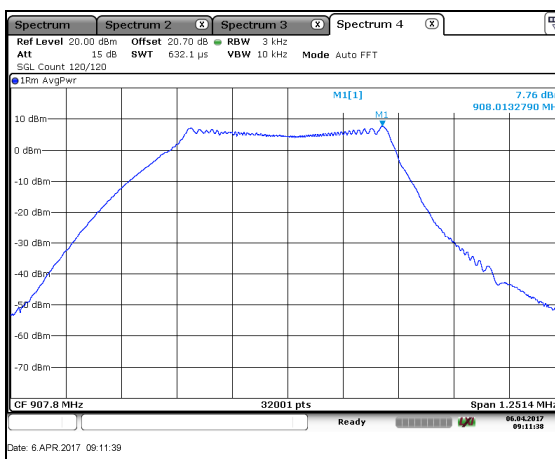
Figure 7.5.2-2: PSD – MCH
