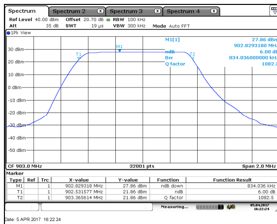
Figure 7.2.2-1: 6dB BW – LCH
