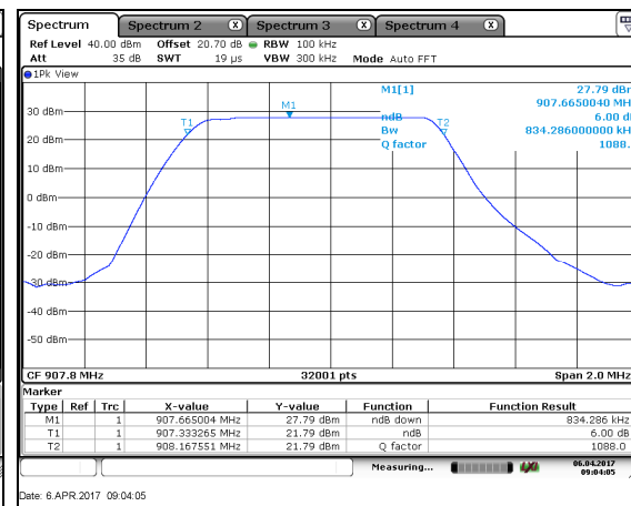
Figure 7.2.2-2: 6dB BW – MCH
