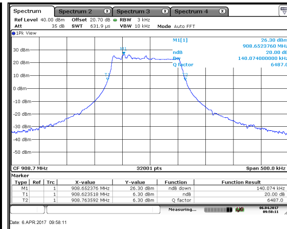
Figure 7.3.4.2-2: 20dB BW Mid Channel
