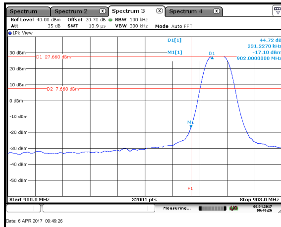
Figure 7.4.1.2-1: Lower Band-Edge
