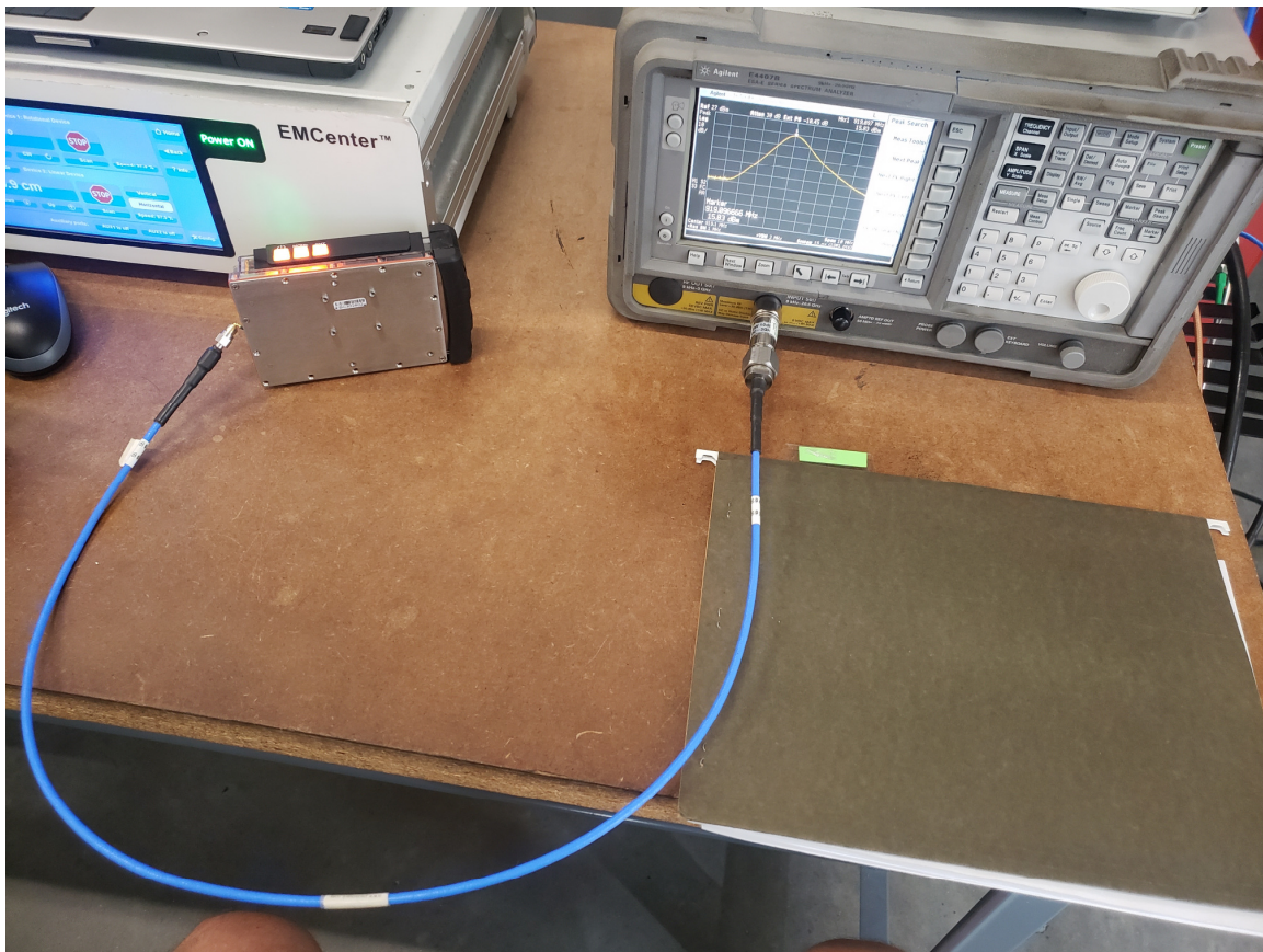
Figure 5. Bench Test Setup
