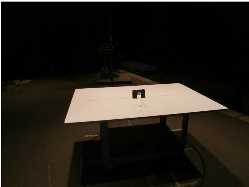
Figure 4: Radiated Emissions – Rear View – YPOS
