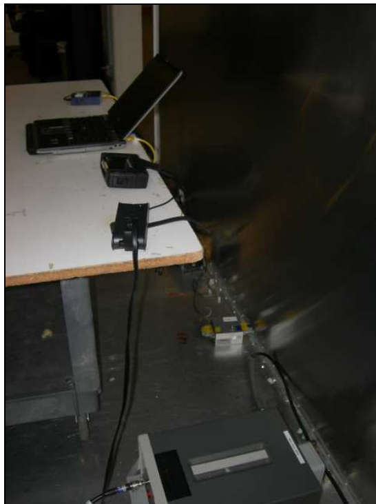
Figure 8: Conducted Emissions – Side View
