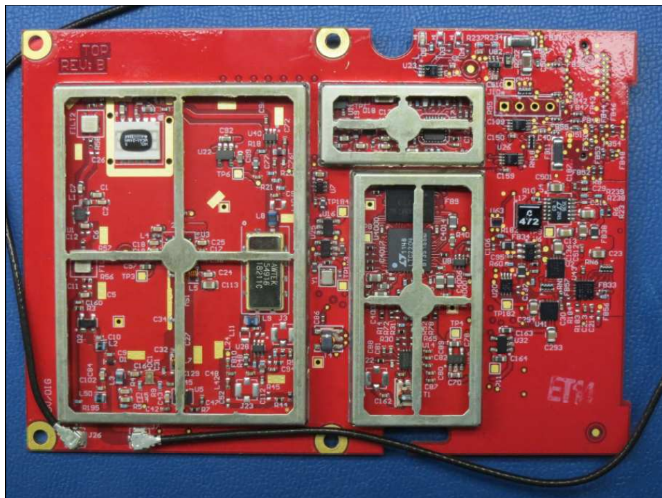
Figure 2: Internal Photo – RF Board Shields Removed
