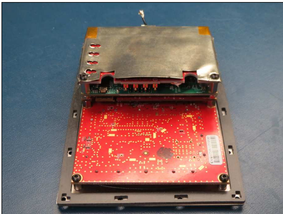
Figure 6: Internal Photo – PCB Assembled
