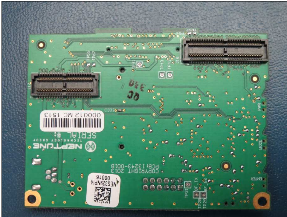
Figure 9: Internal Photo – IO Board
