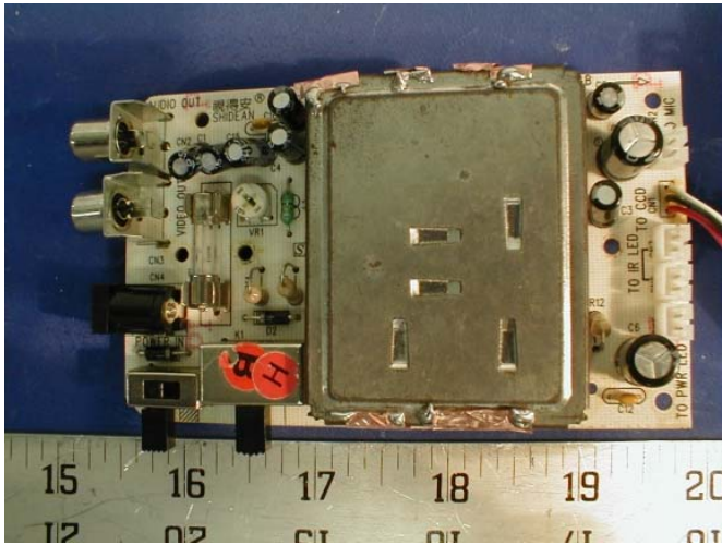
Transmitter – Component View 1
