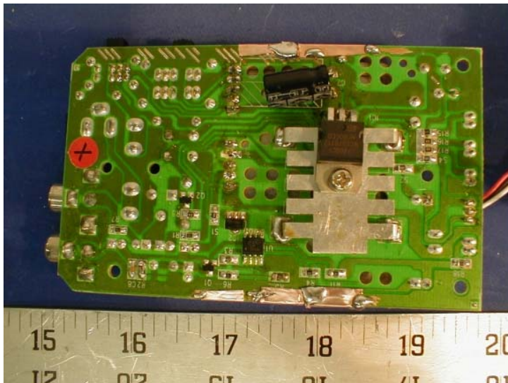
Transmitter – Solder View 1
