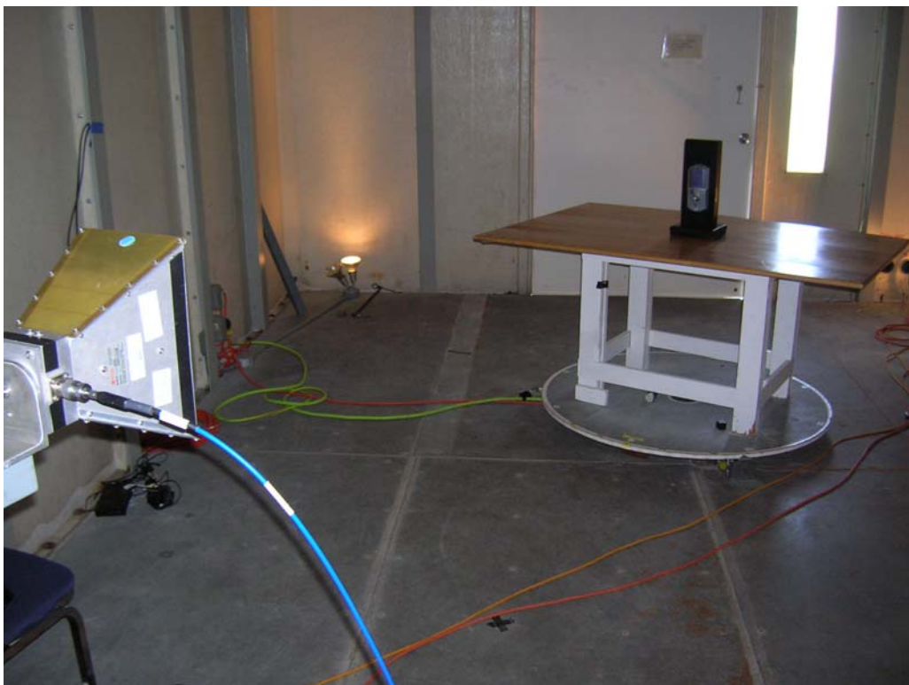
High Frequency Spurious Emissions, Fundamental
