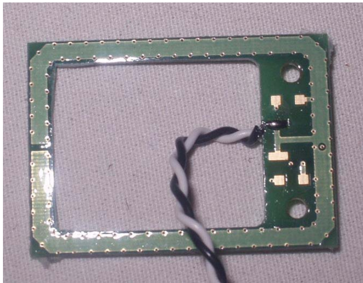
13.56 MHz Card reader Antenna
