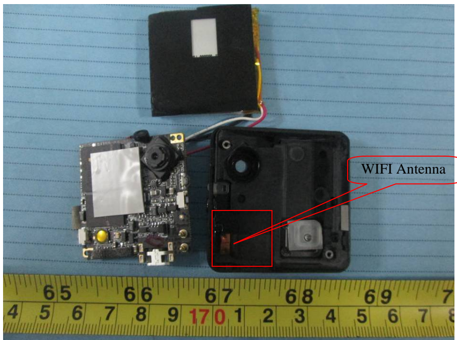
EUT – Cover off View 2 (With Antenna 1: KeXinHuaCheng)
