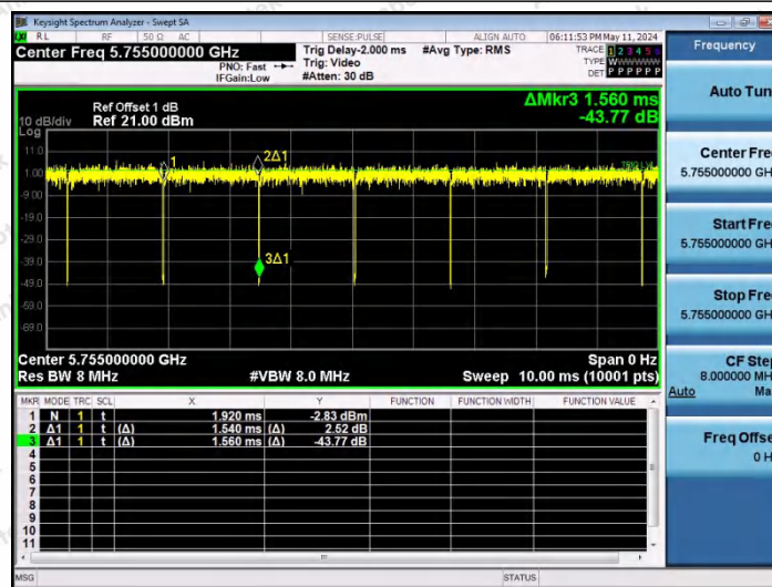
NTNV-11AC40SISO-Ant1-5755
