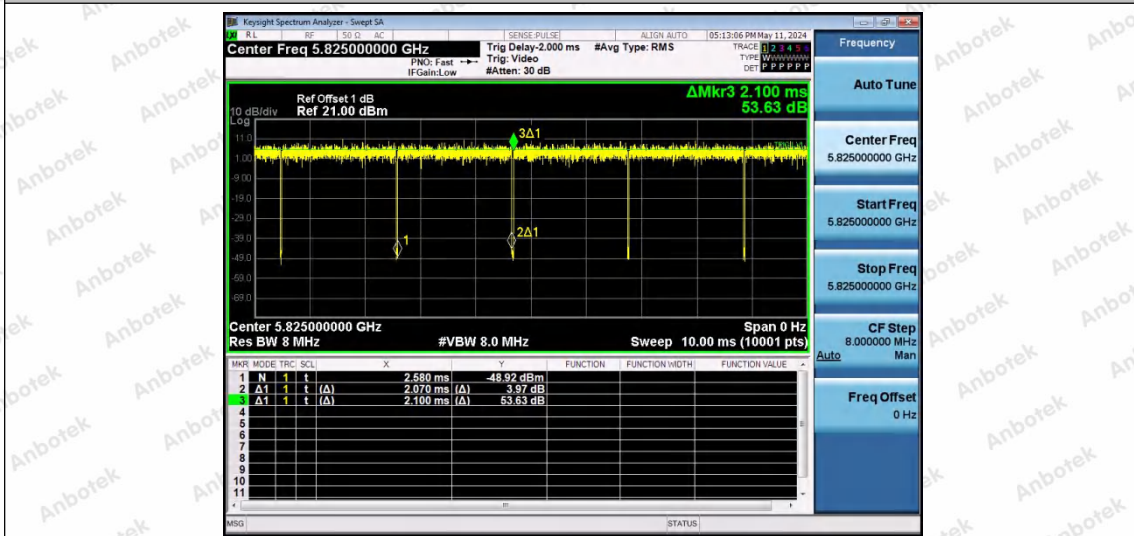
NTNV-11A-Ant1-5825
