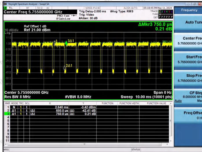
NTNV-11N40SISO-Ant1-5755
