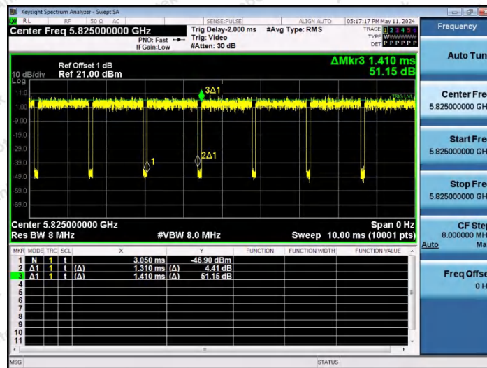
NTNV-11N20SISO-Ant1-5825
