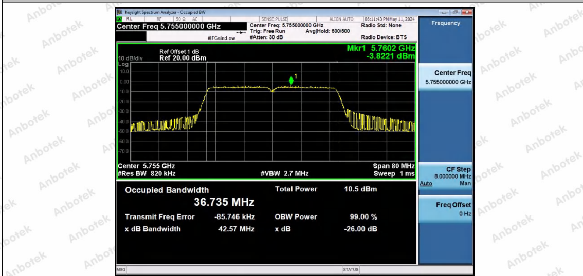
11AC40SISO-Ant1-5755
