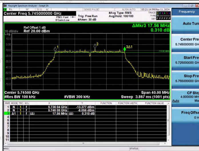
11A20SISO-Ant1-5745-PASS
