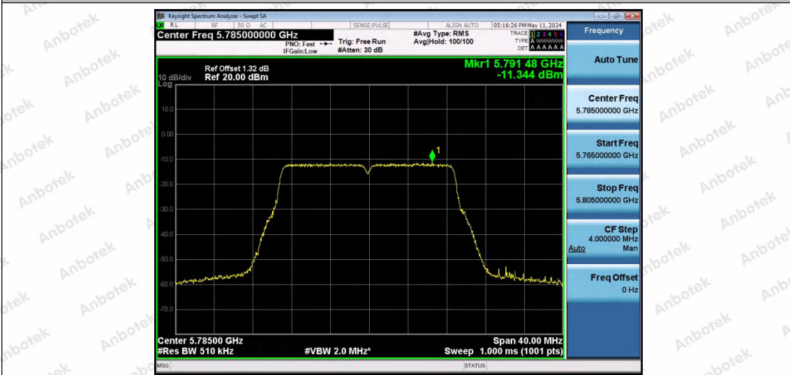
11N20SISO-Ant1-5785-PASS
