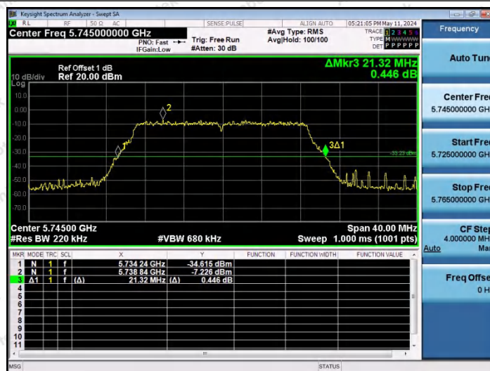
11A20SISO-Ant1-5745
