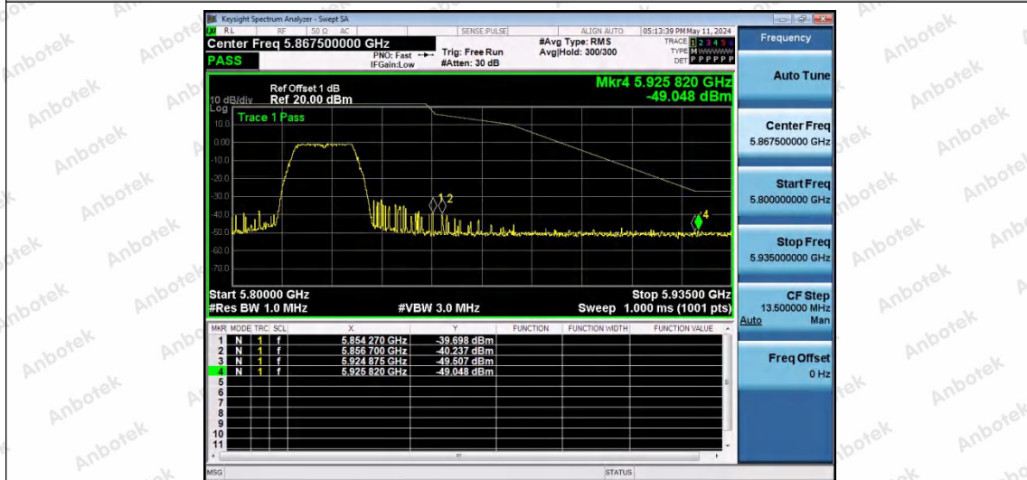
11A-Ant1-5825-PASS
