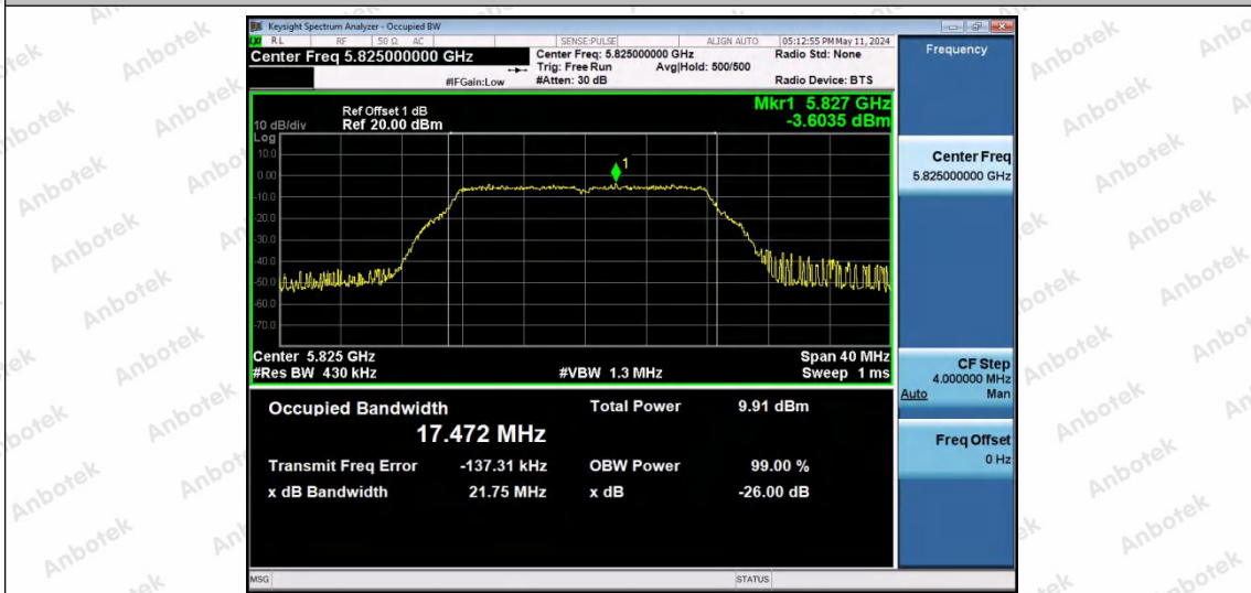
11A-Ant1-5825
