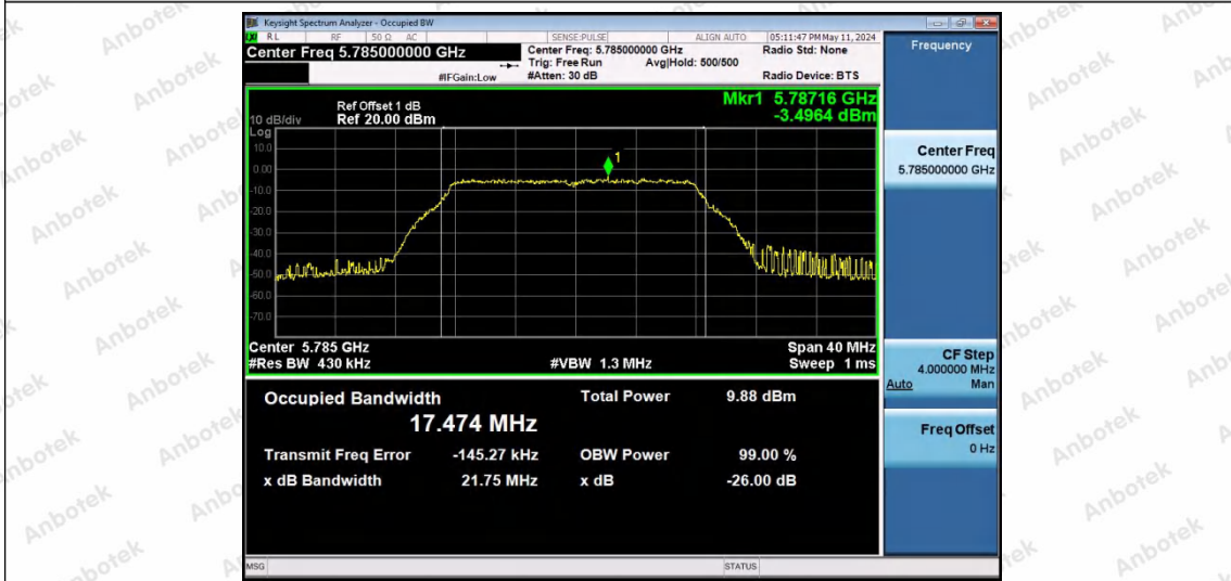
11A-Ant1-5785
