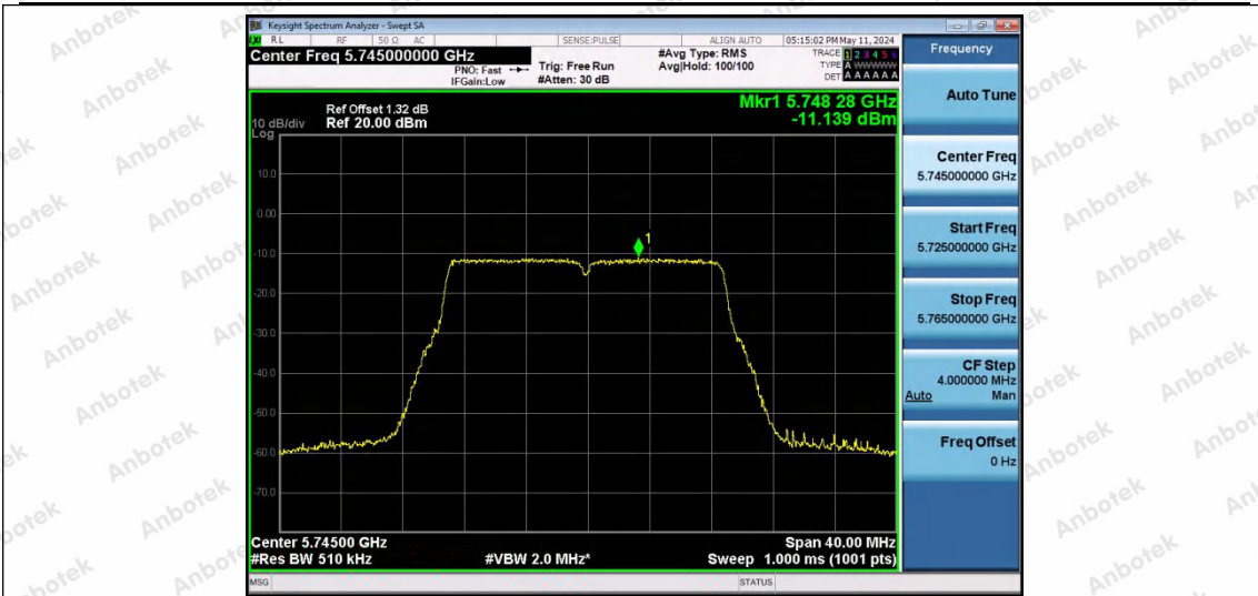
11N20SISO-Ant1-5745-PASS
