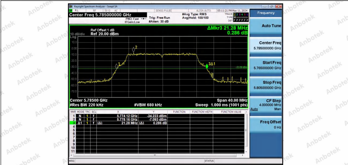
11A-Ant1-5785
