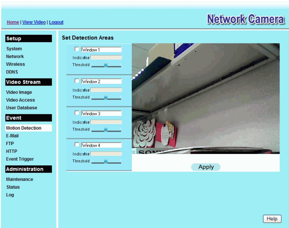
Figure 22: Motion Detection
