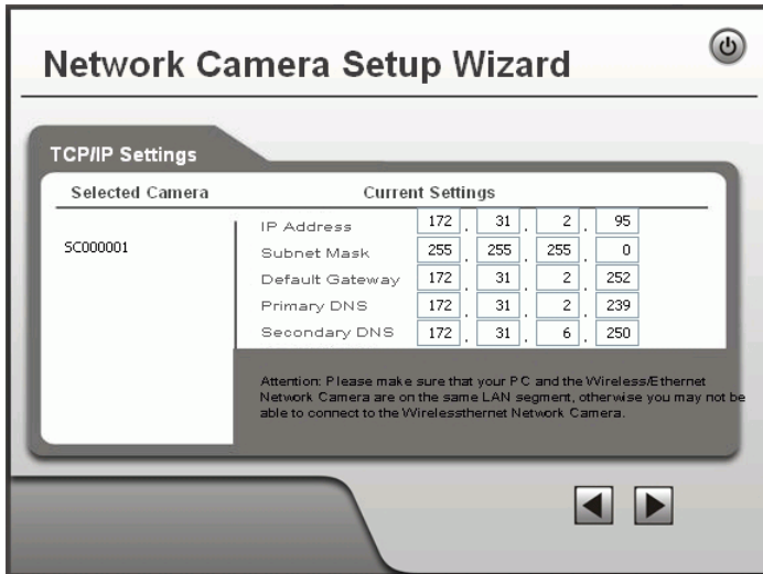
Figure 6: TCP/IP Settings
