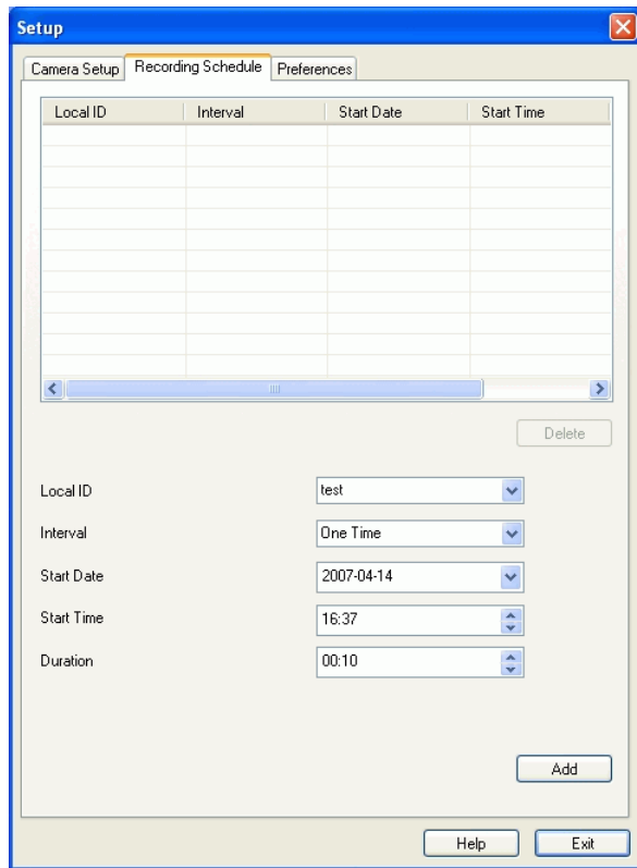
Figure 44: Recording Schedule
