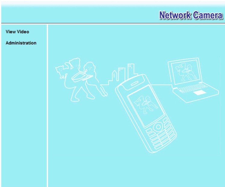
Figure 11: Home Screen
