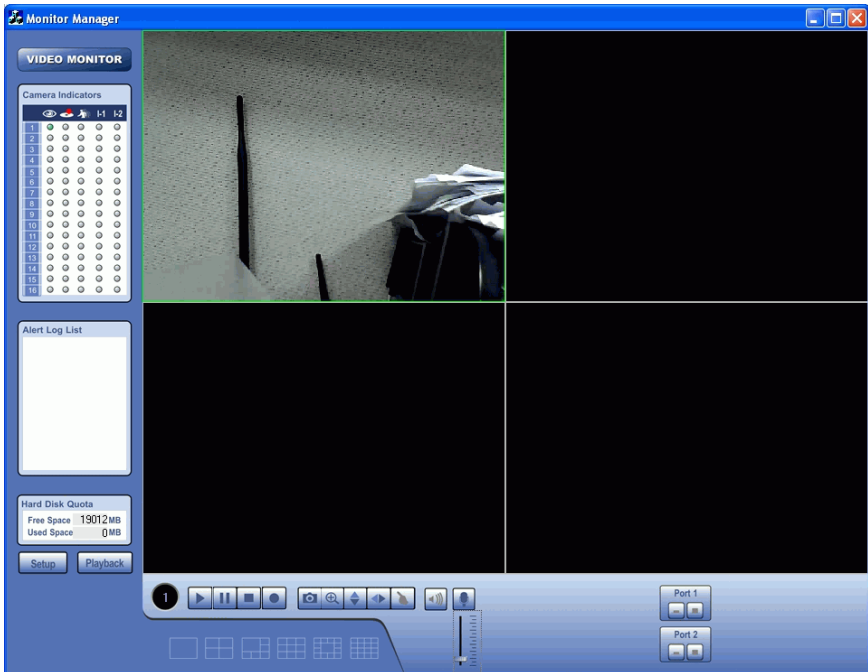
Figure 41: Main Screen
