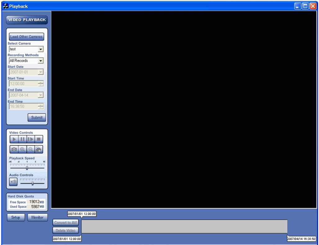
Figure 46: Playback Screen
