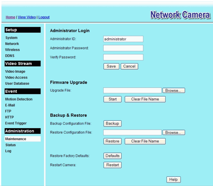
Figure 36: Maintenance Screen
