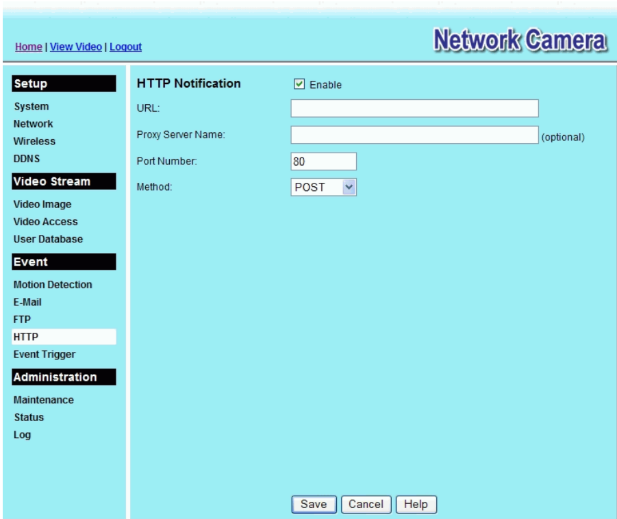
Figure 34: HTTP Screen
