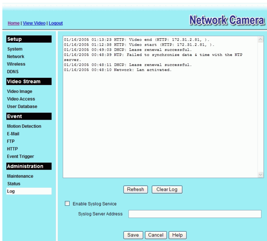
Figure 38: Log Screen
