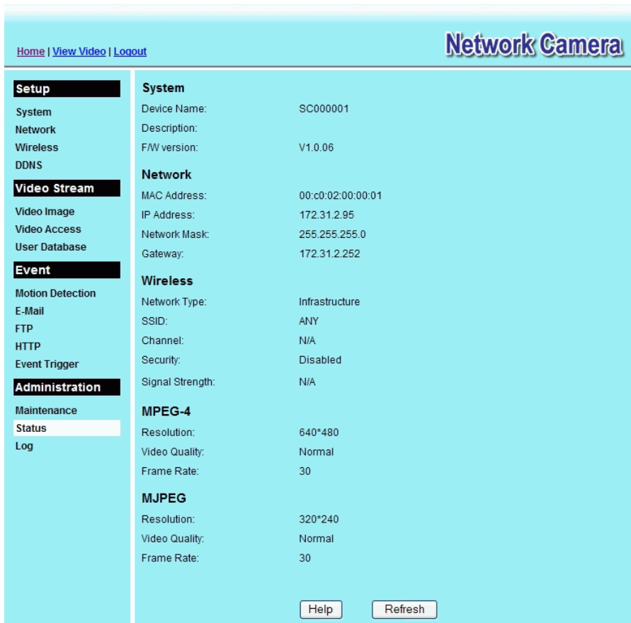
Figure 37: Status Screen
