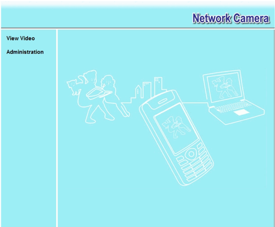
Figure 23: Welcome Screen
