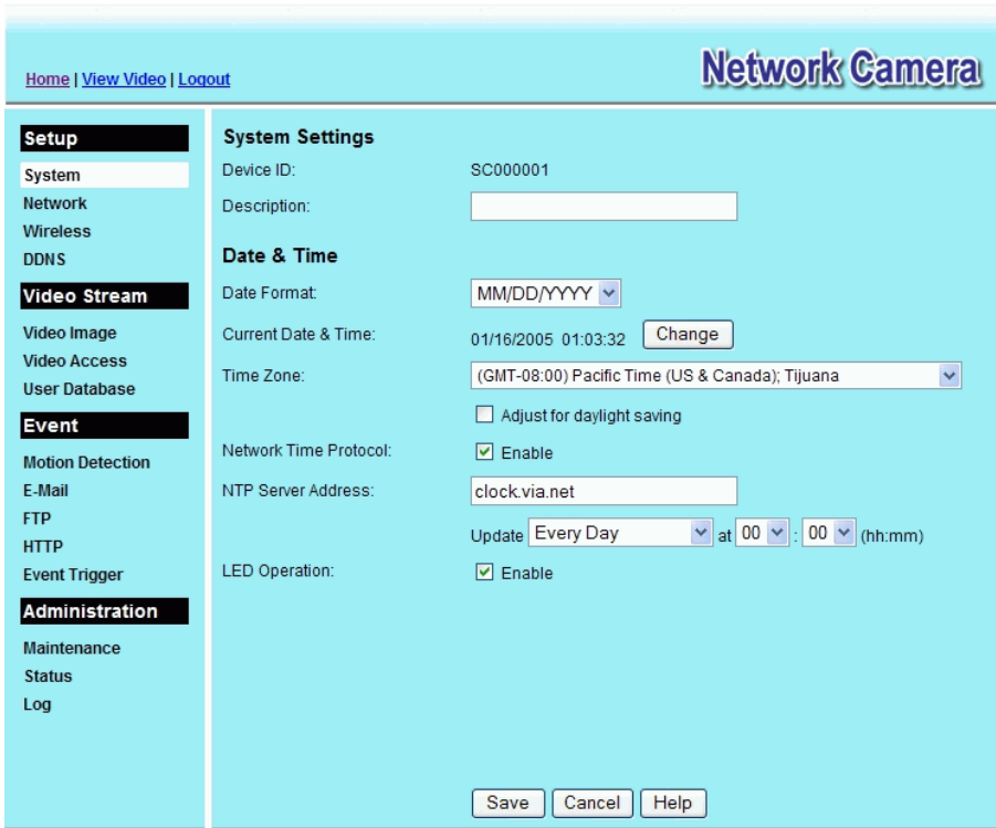
Figure 24: System Screen
