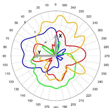
Azimuth XY 5200 MHz
