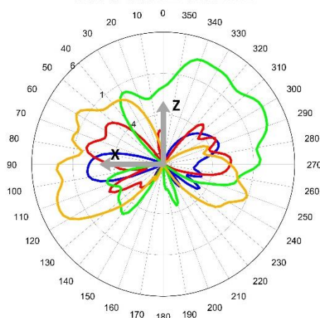
Side to Side XZ 5200 MHz
