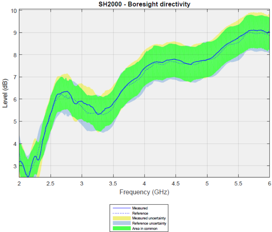
Figure 5.60: Boresight directivity
