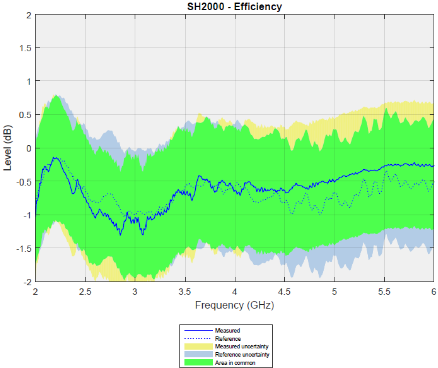
Figure 5.62: Efficiency
