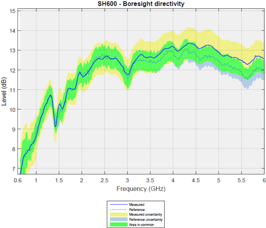
Figure 5.1: Boresight directivity
