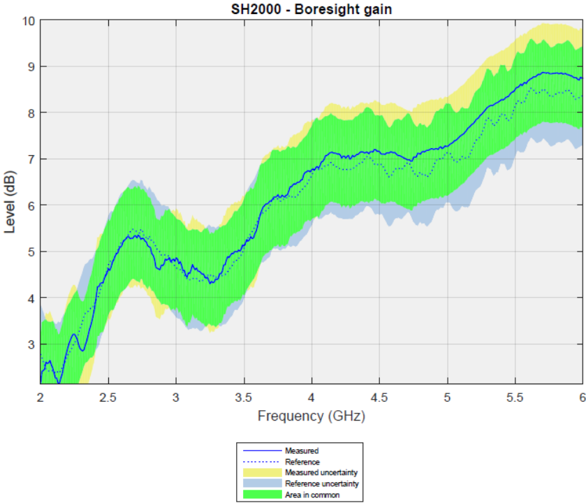
Figure 5.61: Boresight gain
