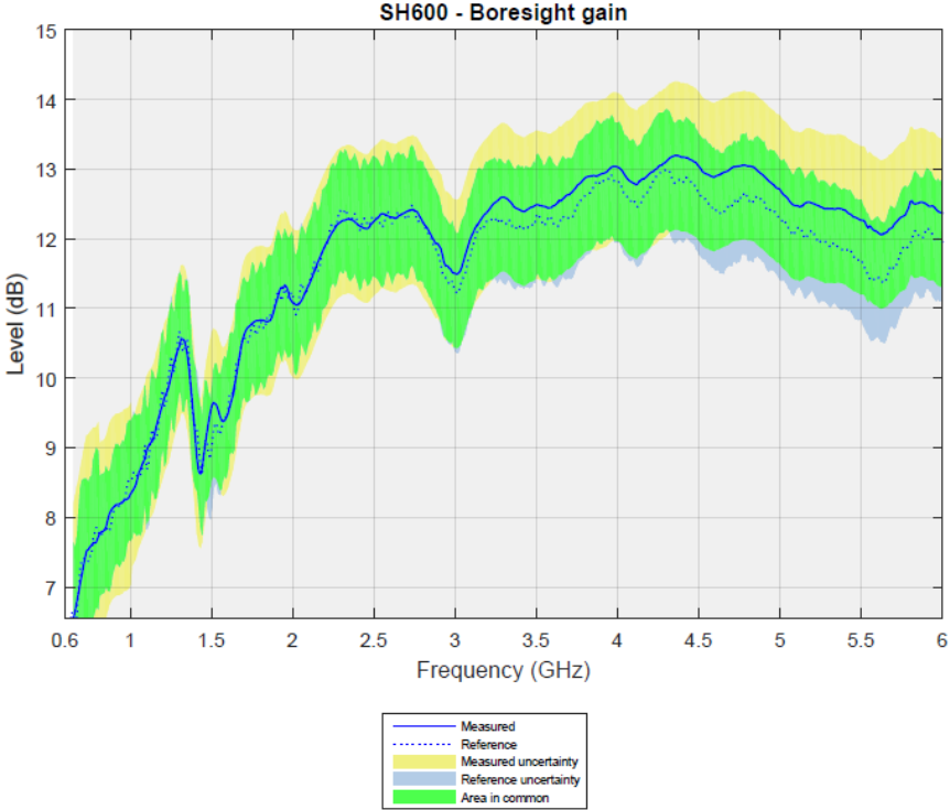
Figure 5.2: Boresight gain
