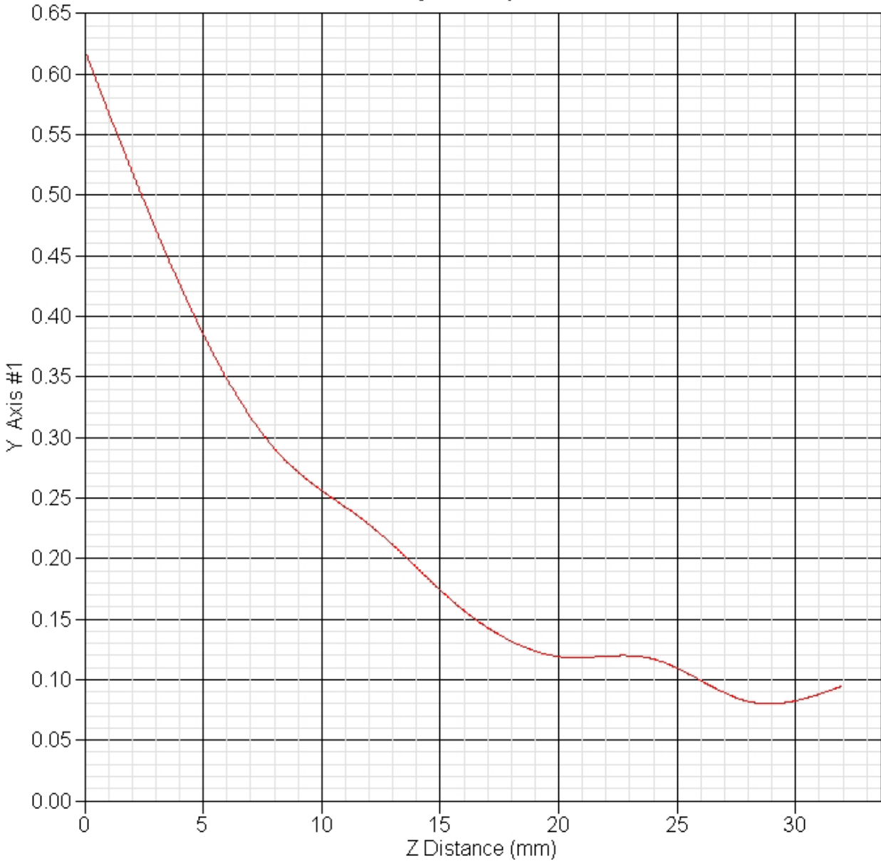
SAR-Z Axis at Hotspot x:20.00 y:-5.00
