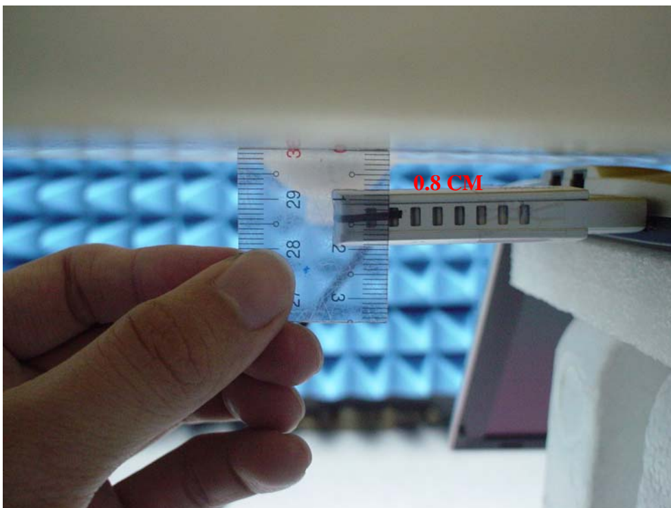
Fig.8 Photograph of the Bottom of the Pc is paralleled and at a distance of 0.0 cm from the base of the phantom, but 0.8 cm Spacing between EUT & Planar Phantom.
