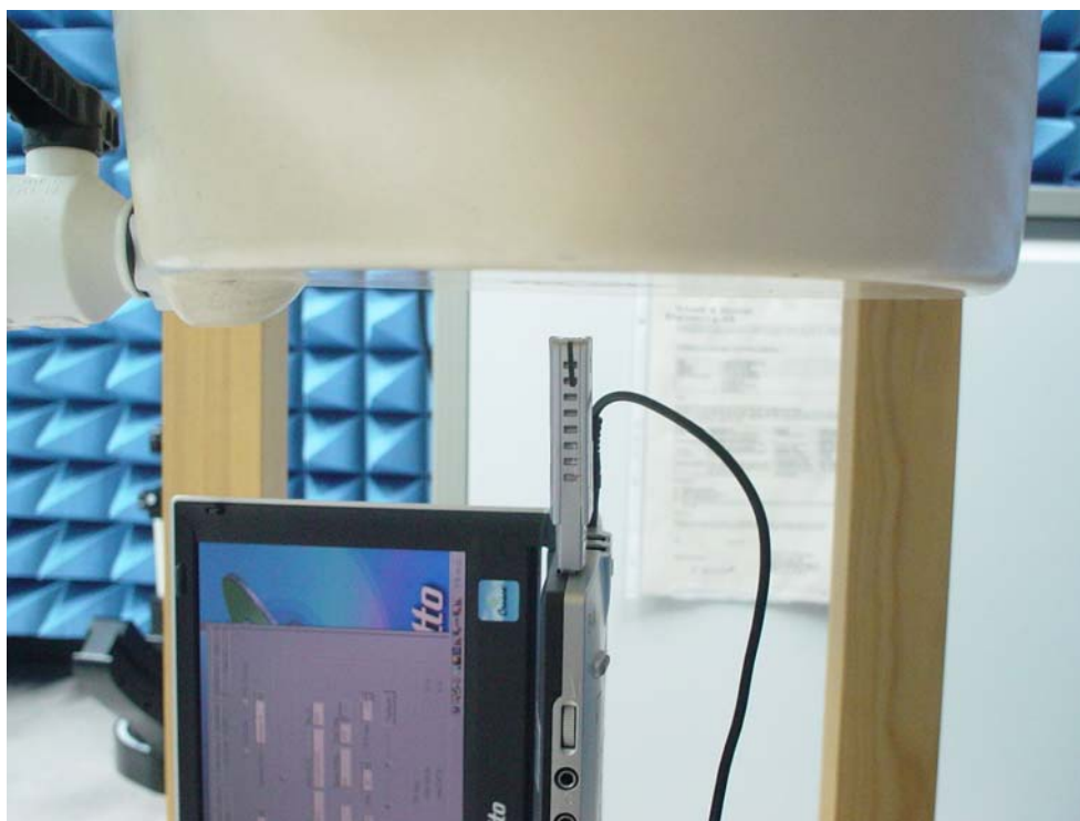
Fig.4 Photograph of the antenna tip is upward and at a distance of 1.5 cm from the base of the phantom.
