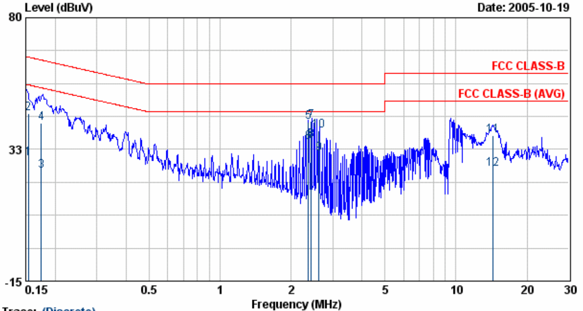
Trace: (Discrete)
