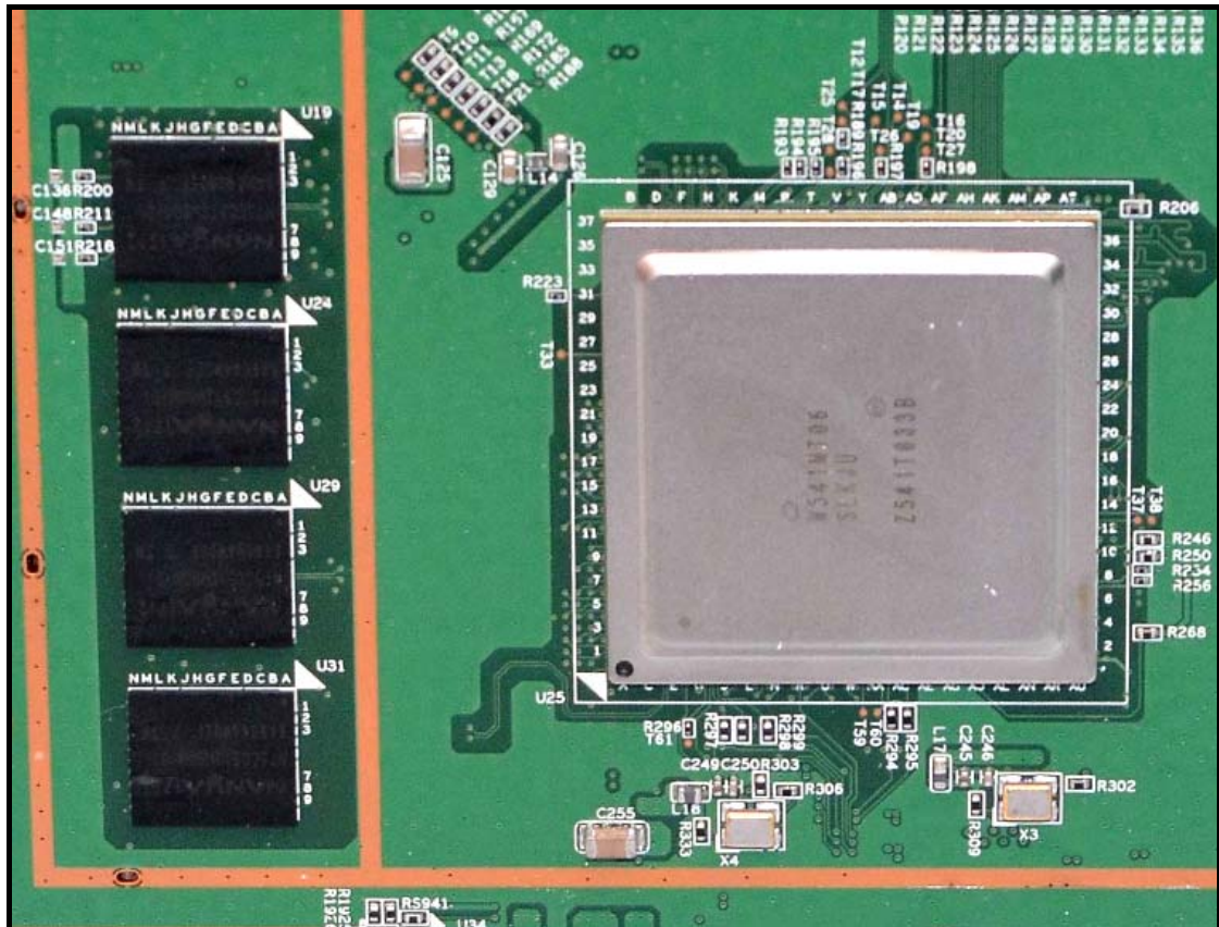
CPU 2
