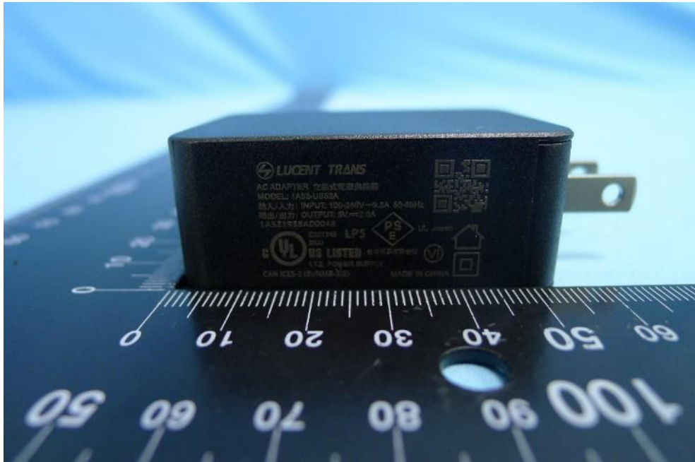
(11) Adapter (1A52-UB52A)
