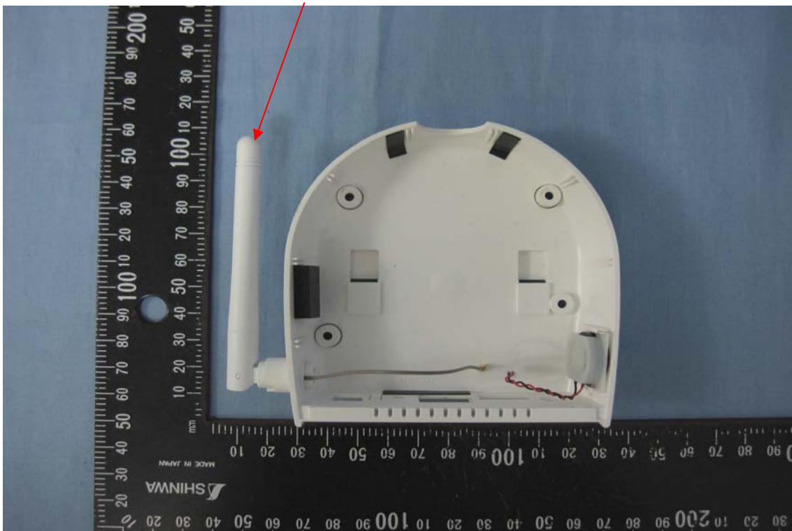
Dipole Antenna
