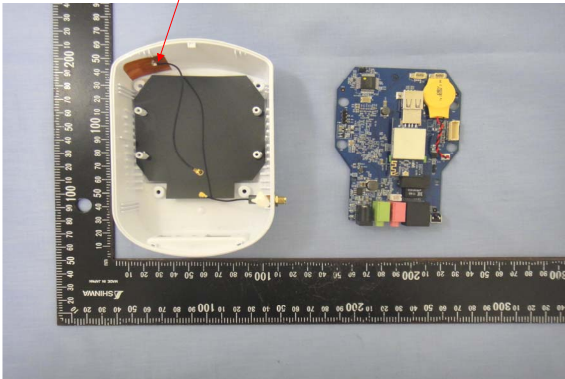
PCB Antenna
