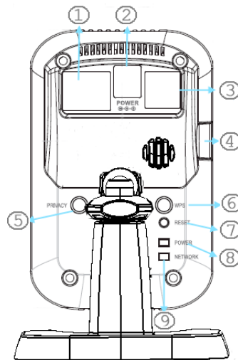
Figure 3: Rear Panel
