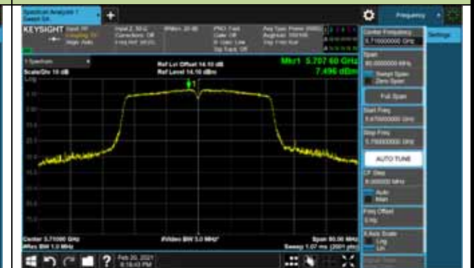
Channel 142 (5710MHz)
