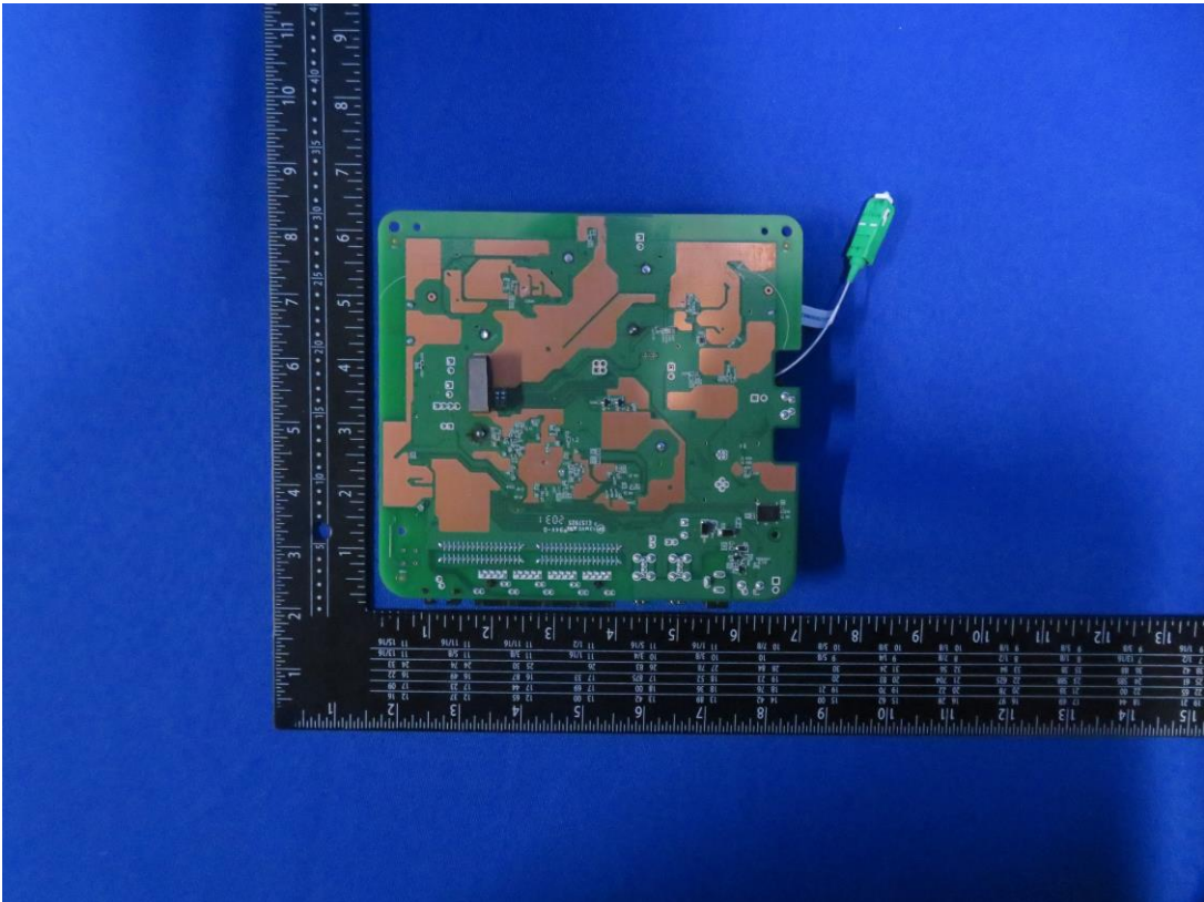
(7) EUT Photo
