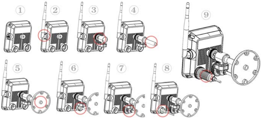
Figure 4: Installing Diagram
