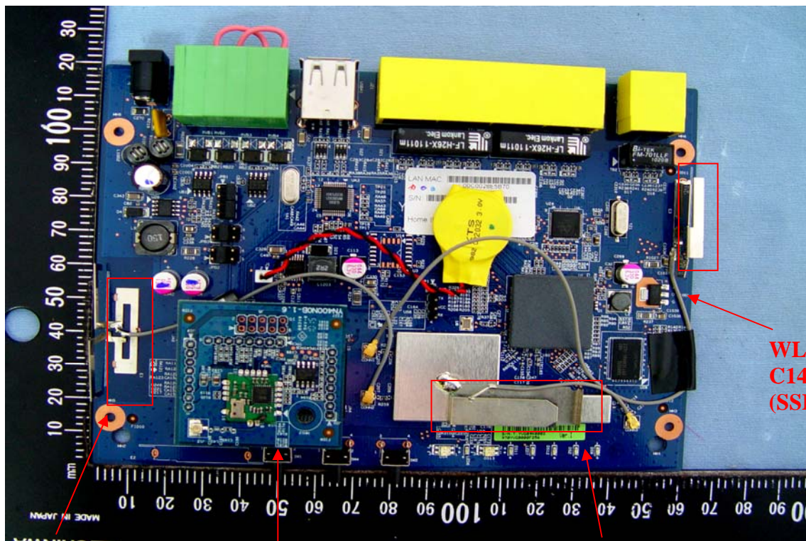
WLAN Antenna C147-510674-A (SSR-210468)
