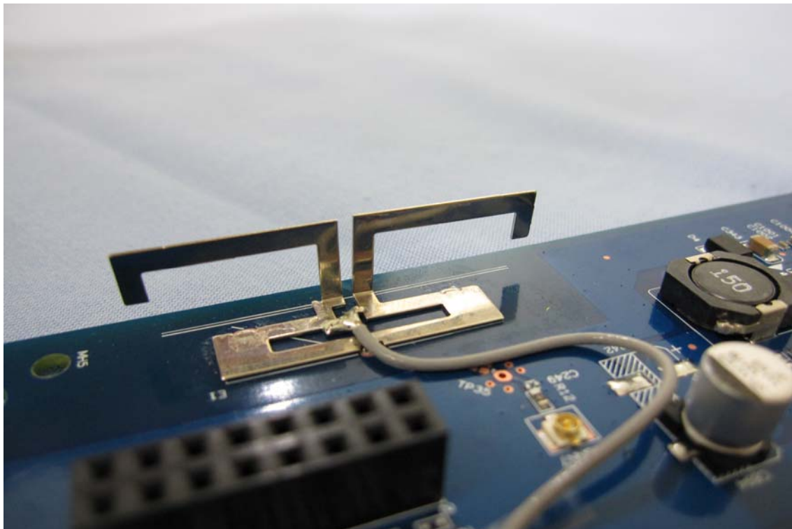
WLAN Antenna
