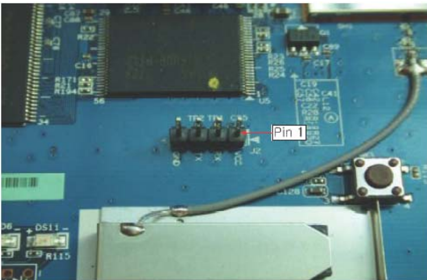
Console port connector
