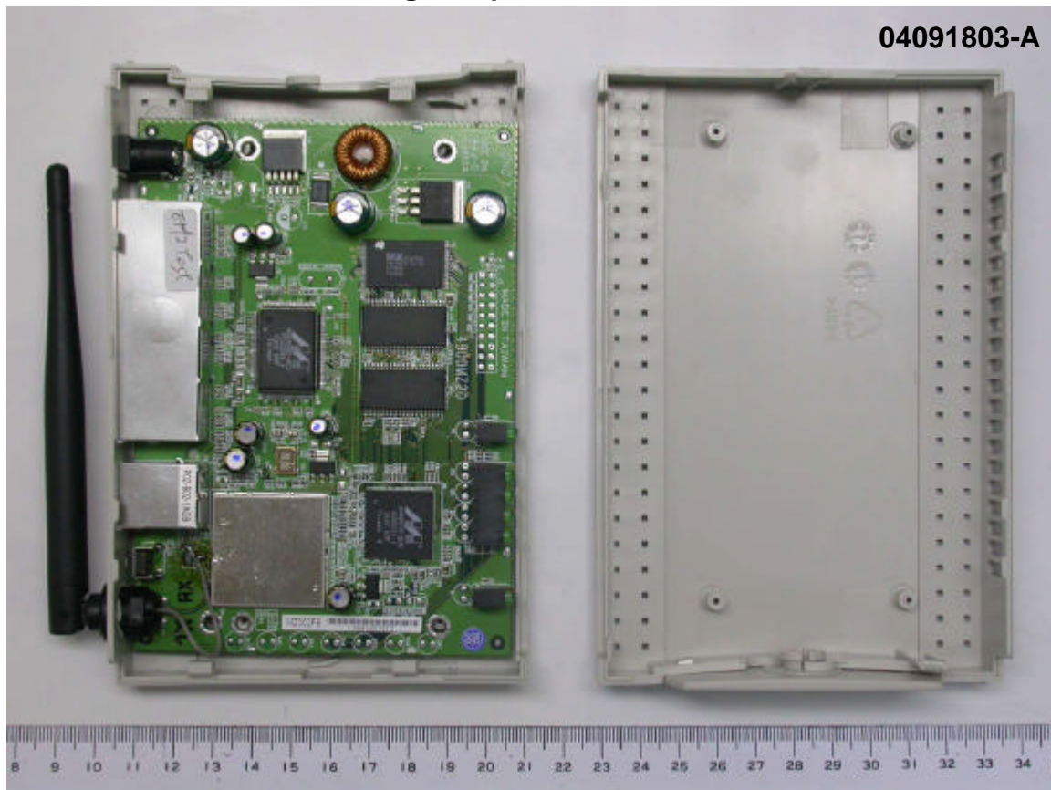
Integral dipole antenna
