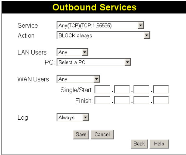
Figure 55: Outbound Services Screen
