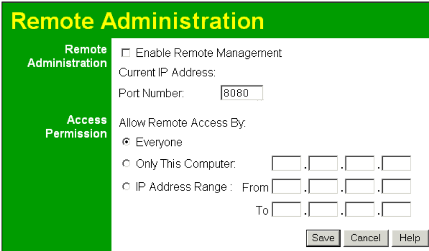
Figure 72: Remote Administration Screen
