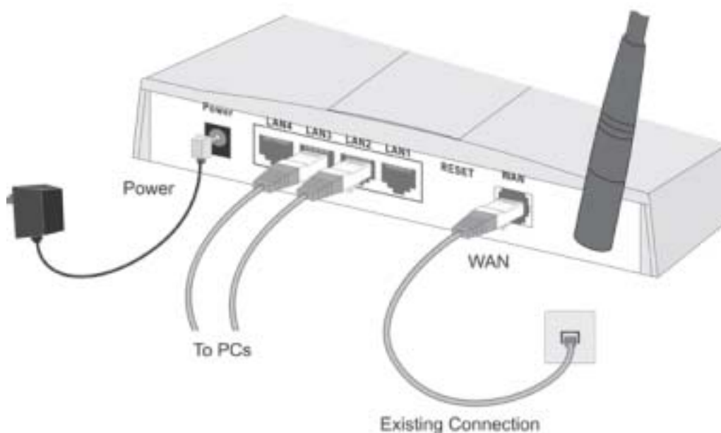
Figure 4: Installation Diagram
