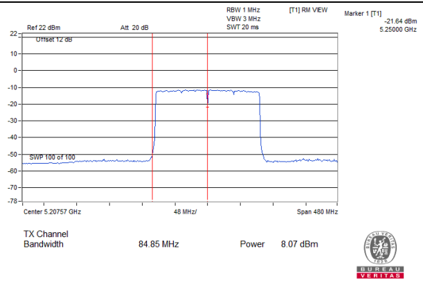
802.11ax (HE160)_Chain 2: CH 50 (For U-NII-1)
