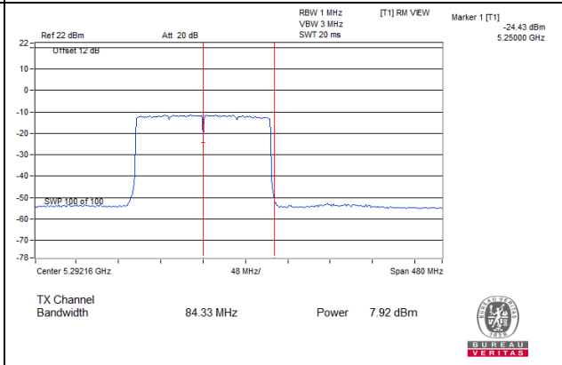
802.11ax (HE160)_Chain 2: CH 50(For U-NII-2A)
