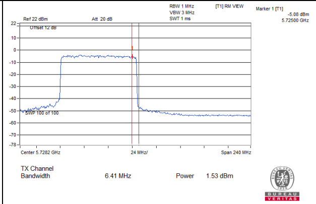
802.11ax (HE80)_Chain 1: CH 138(For U-NII-3)
