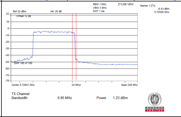
802.11ax (HE80)_Chain 3: CH 138(For U-NII-3)
