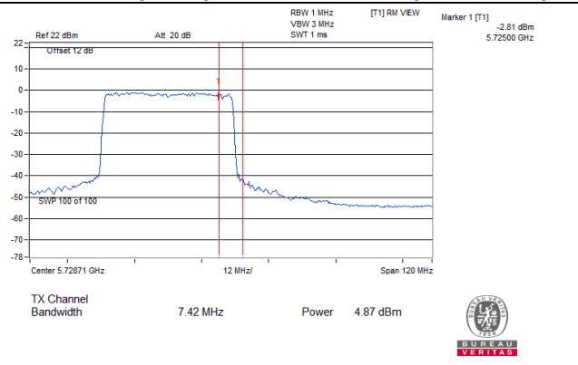
802.11ax (HE40)_Chain 3: CH 142(For U-NII-3)
