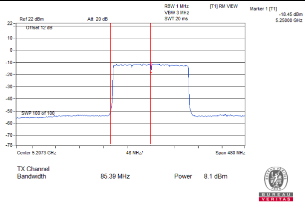
802.11ax (HE160)_Chain 1: CH 50 (For U-NII-1)
