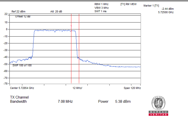
802.11ax (HE40)_Chain 2: CH 142(For U-NII-3)
