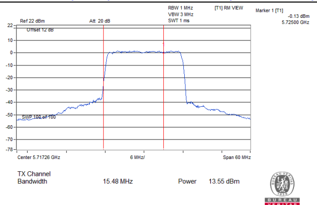
802.11ax (HE20)_Chain 3: CH 144 (For U-NII-2C)
