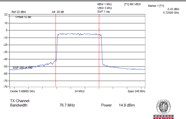
802.11ax (HE80)_Chain 2: CH 138 (For U-NII-2C)
