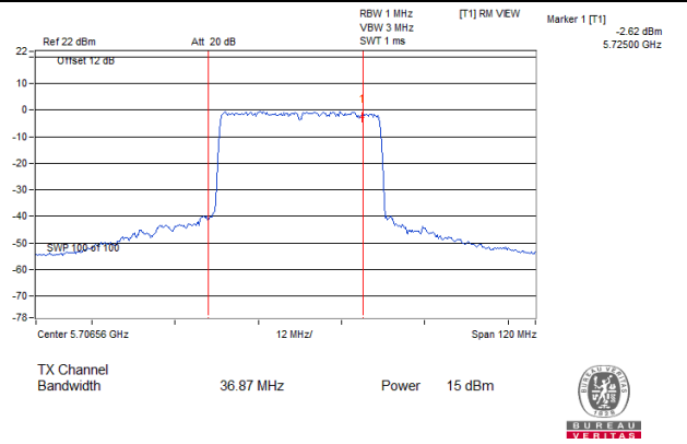
802.11ax (HE40)_Chain 1: CH 142 (For U-NII-2C)
