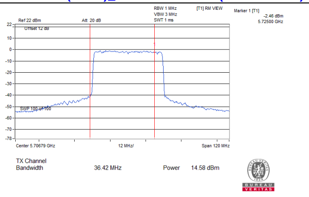
802.11ax (HE40)_Chain 3: CH 142 (For U-NII-2C)
