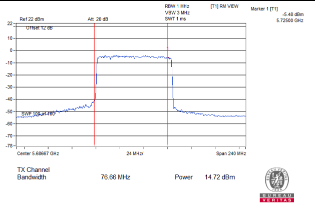
802.11ax (HE80)_Chain 1: CH 138 (For U-NII-2C)
