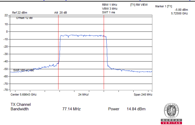
802.11ax (HE80)_Chain 3: CH 138 (For U-NII-2C)
