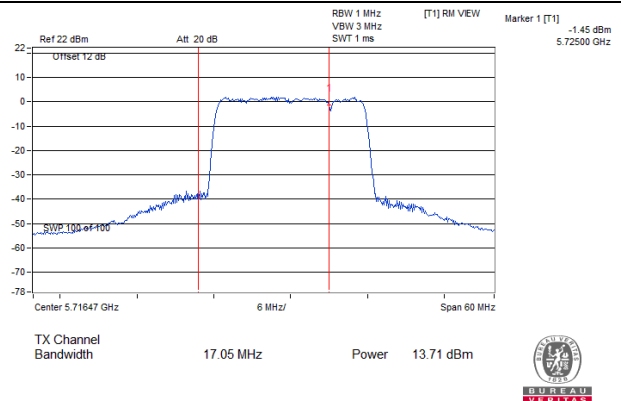
802.11ax (HE20)_Chain 2: CH 144 (For U-NII-2C)
