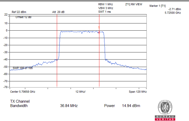
802.11ax (HE40)_Chain 2: CH 142 (For U-NII-2C)
