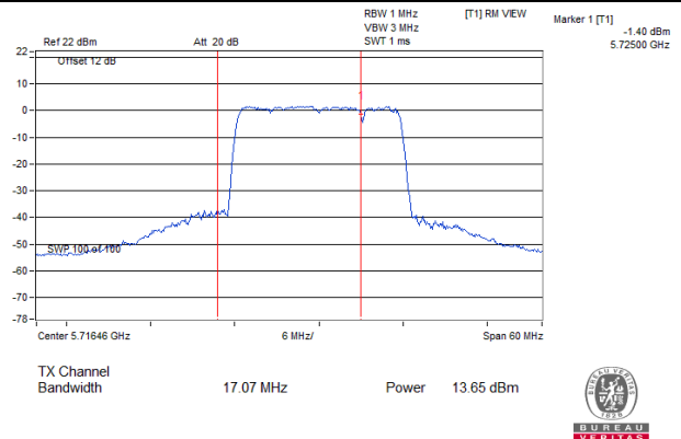
802.11ax (HE20)_Chain 1: CH 144 (For U-NII-2C)
