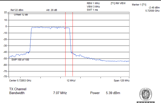
802.11ax (HE40)_Chain 1: CH 142(For U-NII-3)
