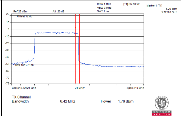
802.11ax (HE80)_Chain 2: CH 138(For U-NII-3)
