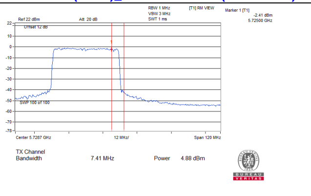
802.11ax (HE40)_Chain 3: CH 142(For U-NII-3)
