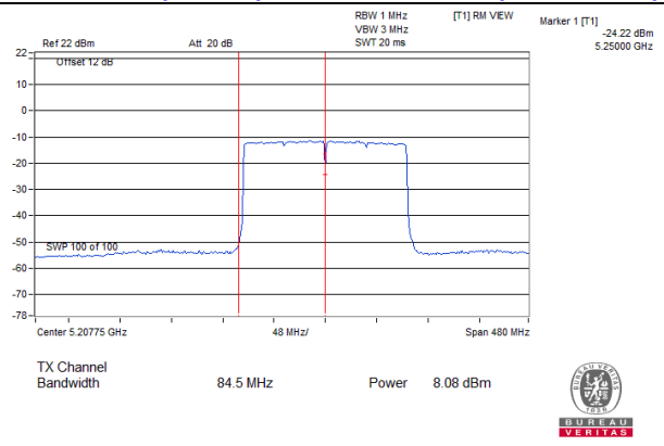
802.11ax (HE160)_Chain 3: CH 50 (For U-NII-1)
