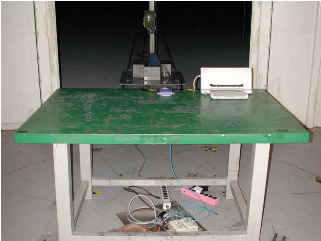
Front View of Radiated Test (Mode 2-Horn)
