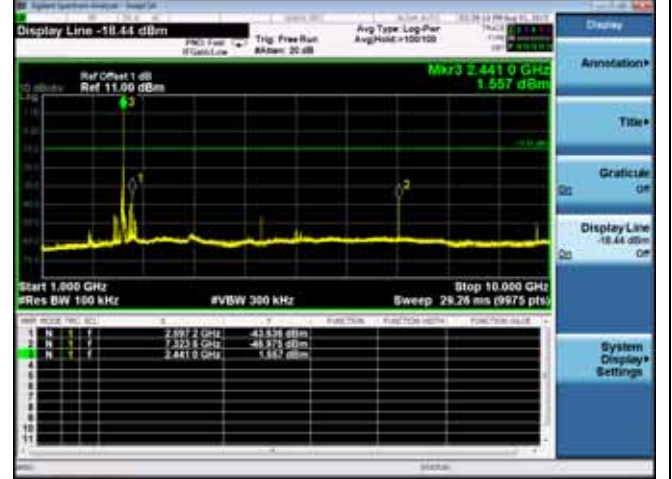
2441MHz(1GHz – 10GHz)
