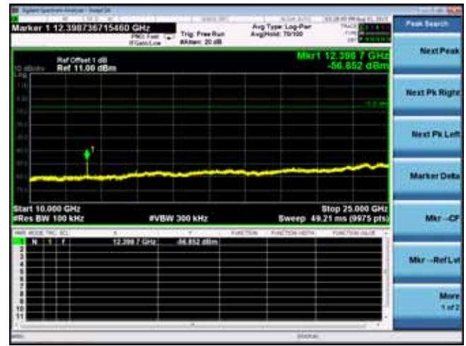
2480MHz(10GHz – 25GHz)
