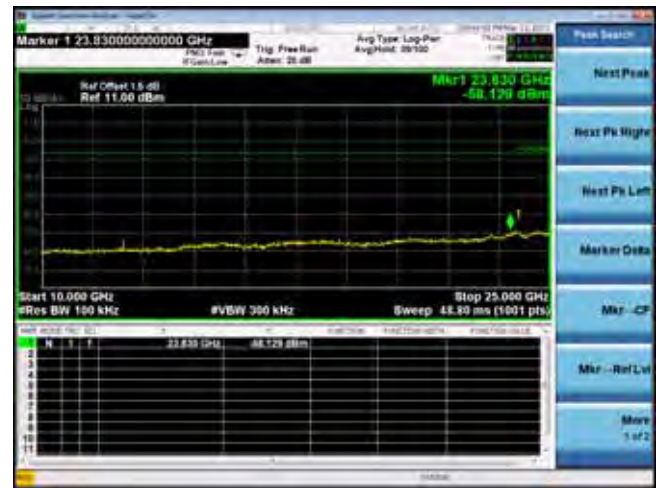
2480MHz(10GHz – 25GHz)
