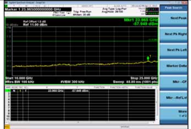
2441MHz(10GHz – 25GHz)
