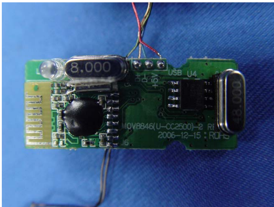
Figure 7 Main Board, Component Side
