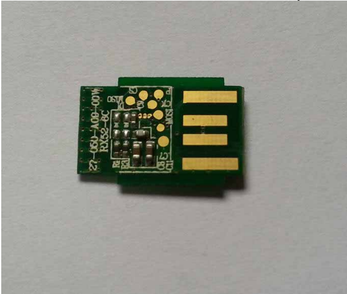
Figure 9 Components Side of the PCB
