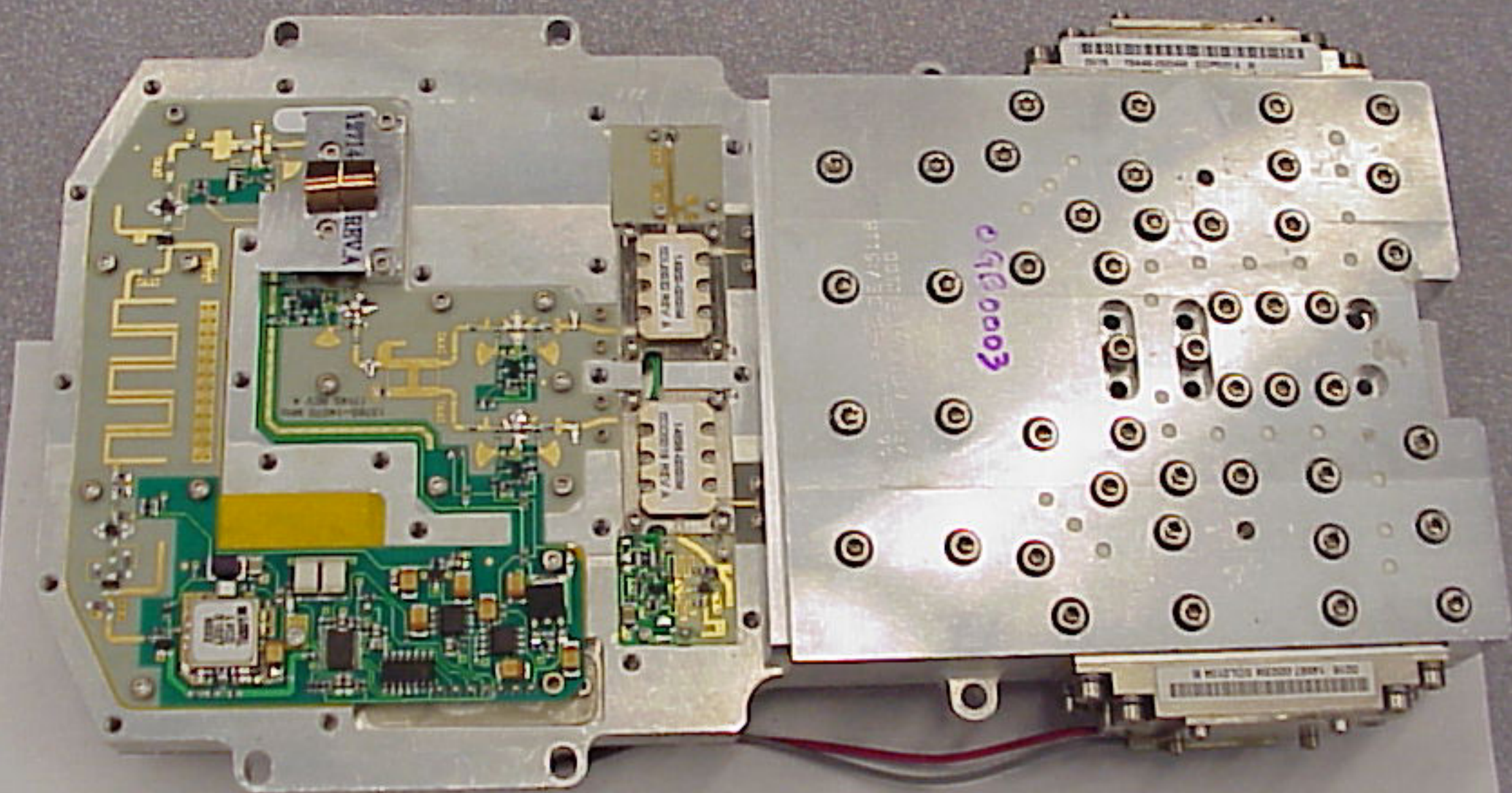
AirStar 39G TX Path
