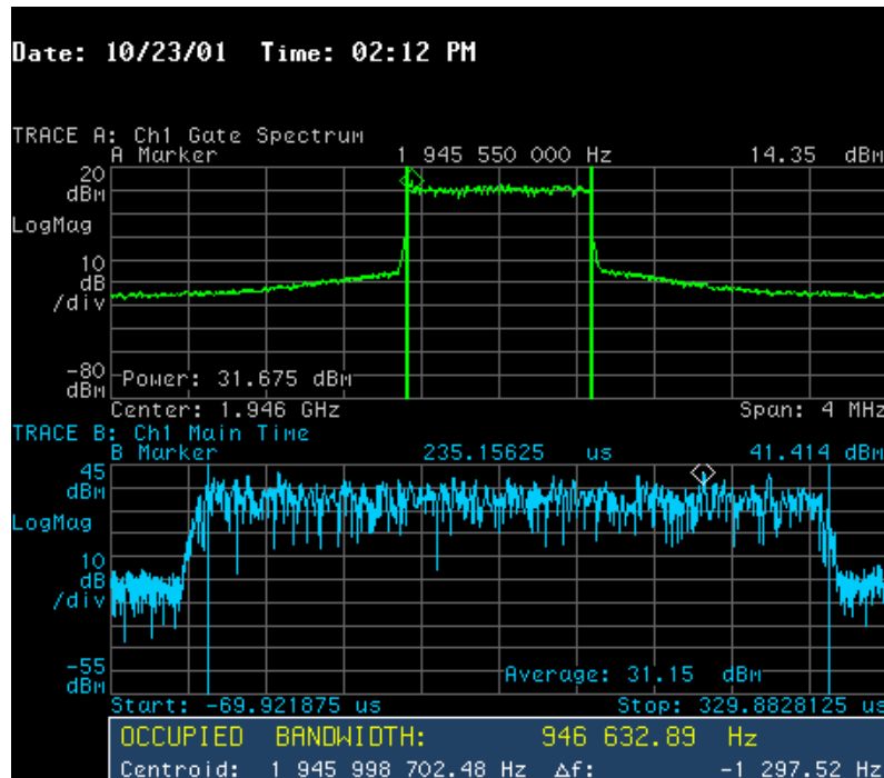
Figure 11.19 High-Speed Data Traffic Channel Power vs. Frequency, 99.0% Occupied BW, and Time-Domain Average Burst Power.
