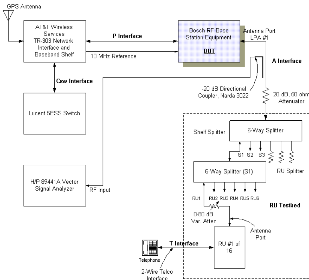
Figure 11.6 Base Station Output Power Test Configuration.
