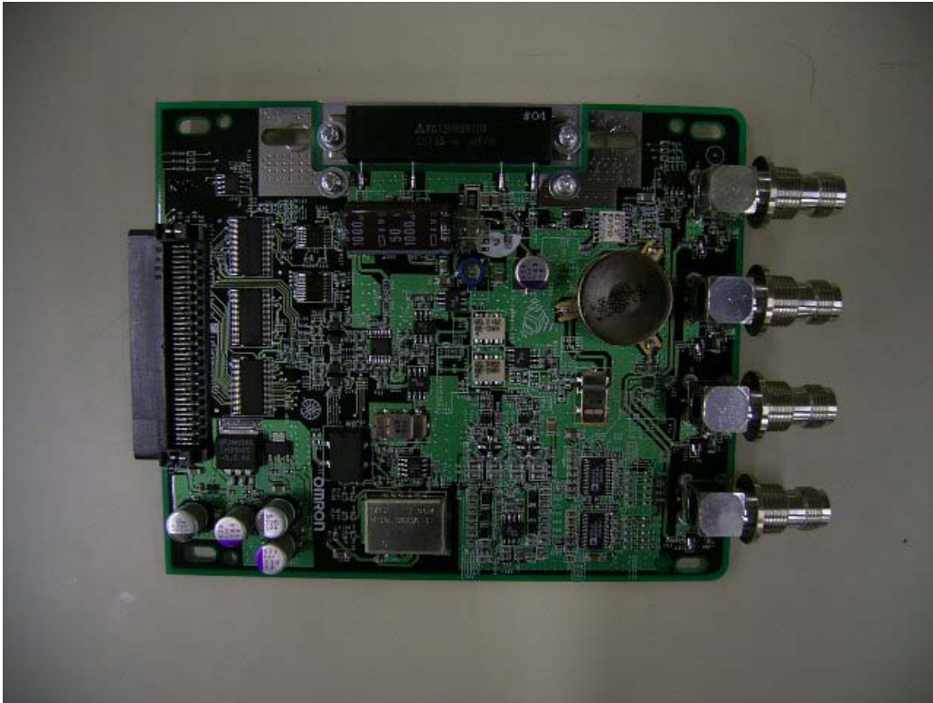
Top of Analog Board
