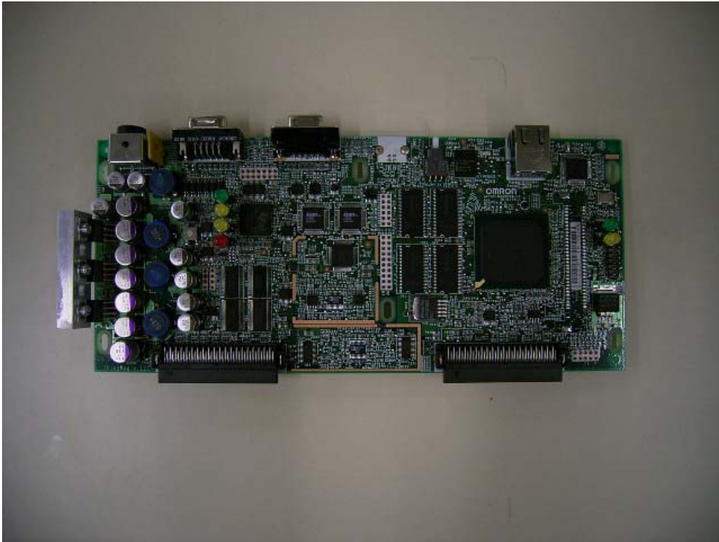
Top of Digital Board
