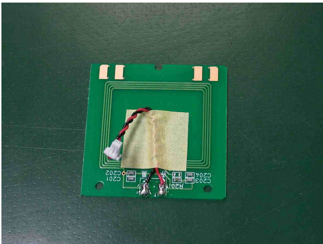
Antenna PCB
