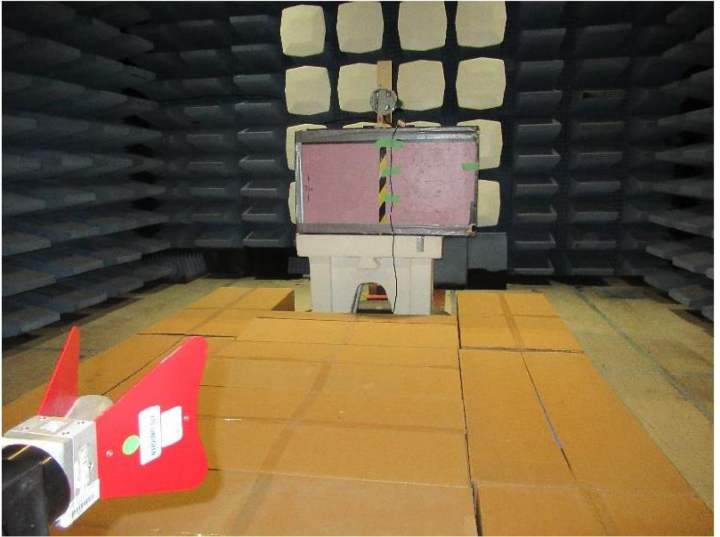
Emissions Test Setup – Intentional Radiated Emissions 1 – 10GHz
