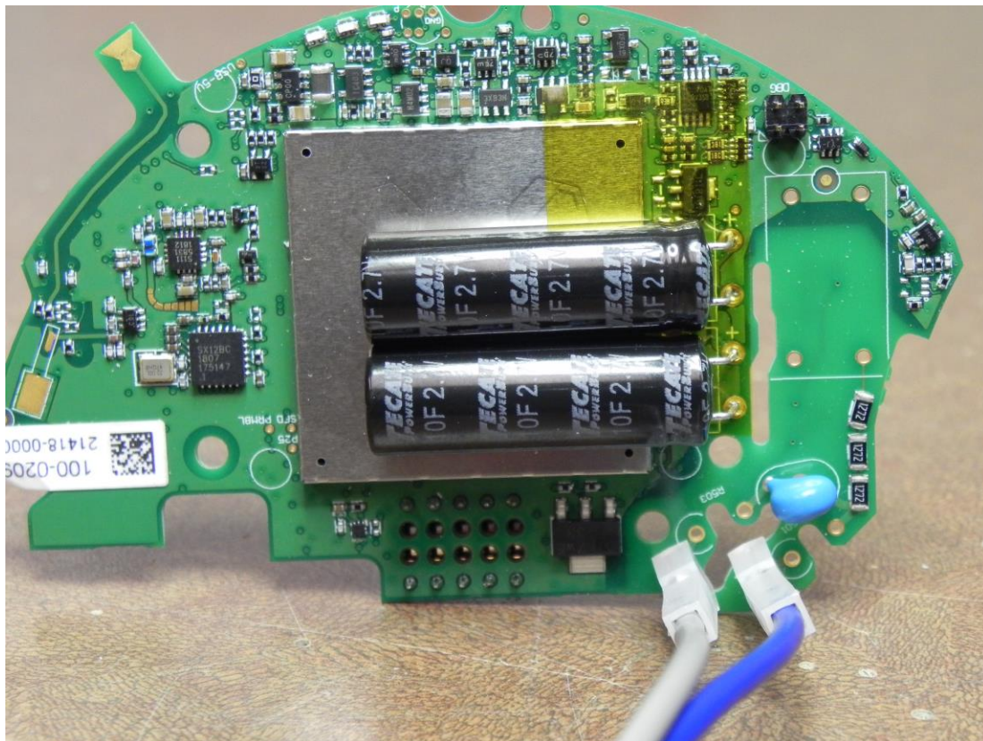
COMMUNICATION MODULE - BOTTOM VIEW (With Shield)
