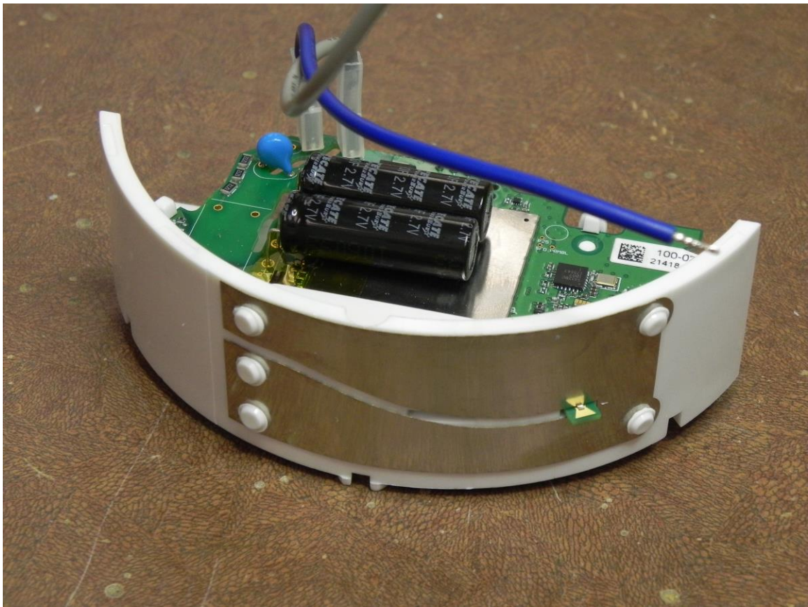
COMMUNICATION MODULE WITH ANTENNA
