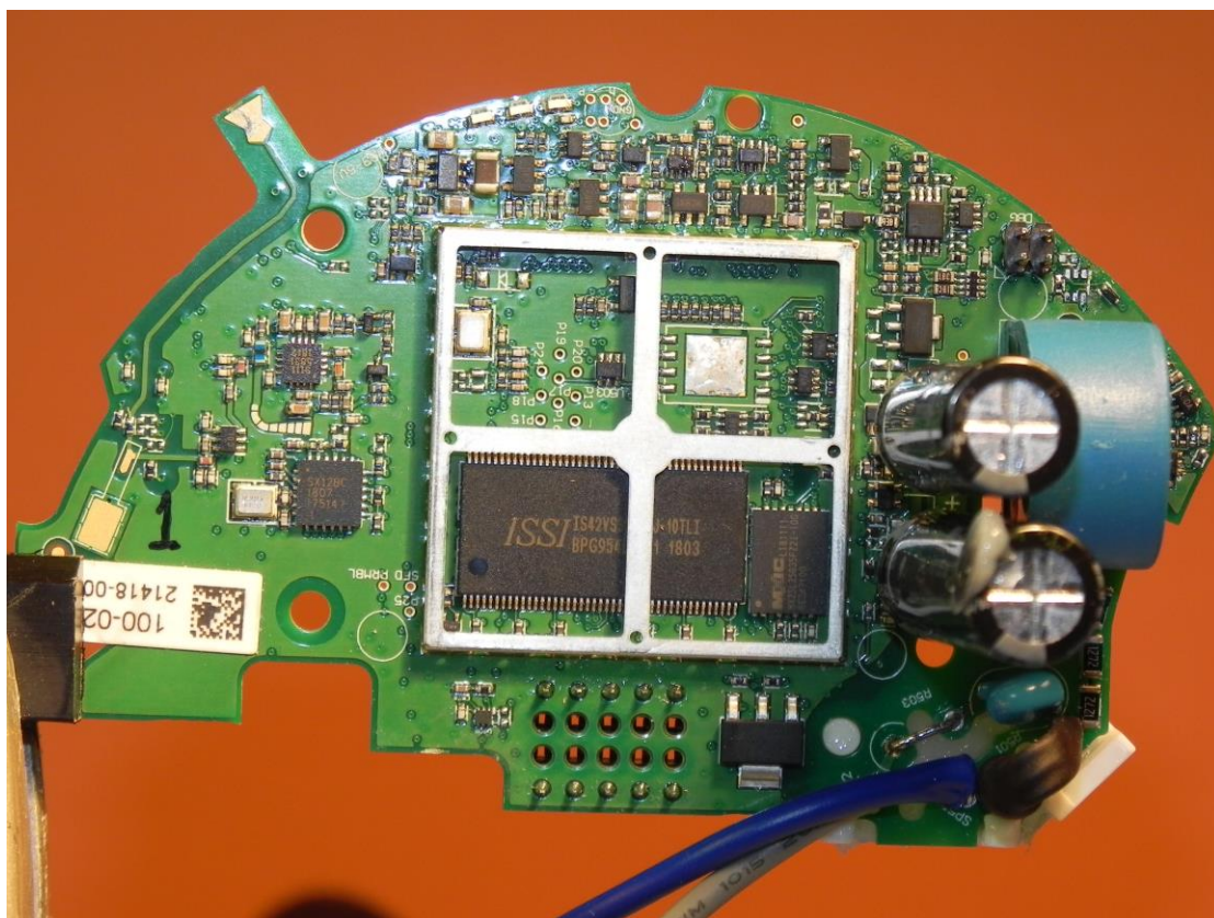
COMMUNICATION MODULE - BOTTOM VIEW (Without Shield)
