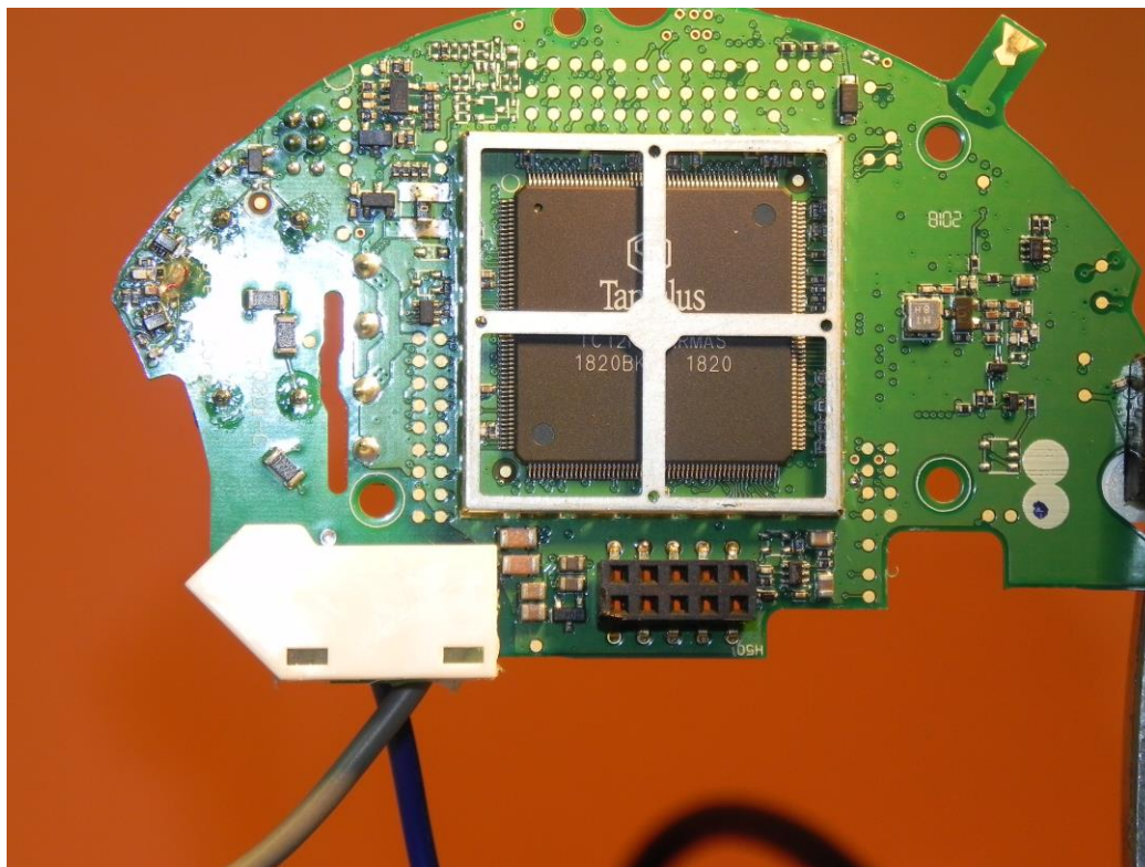
COMMUNICATION MODULE – TOP VIEW (Without Shield)
