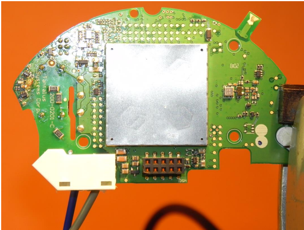
COMMUNICATION MODULE – TOP VIEW (With Shield)
