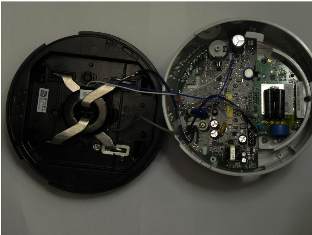
Internal View – Communication Module Attached
