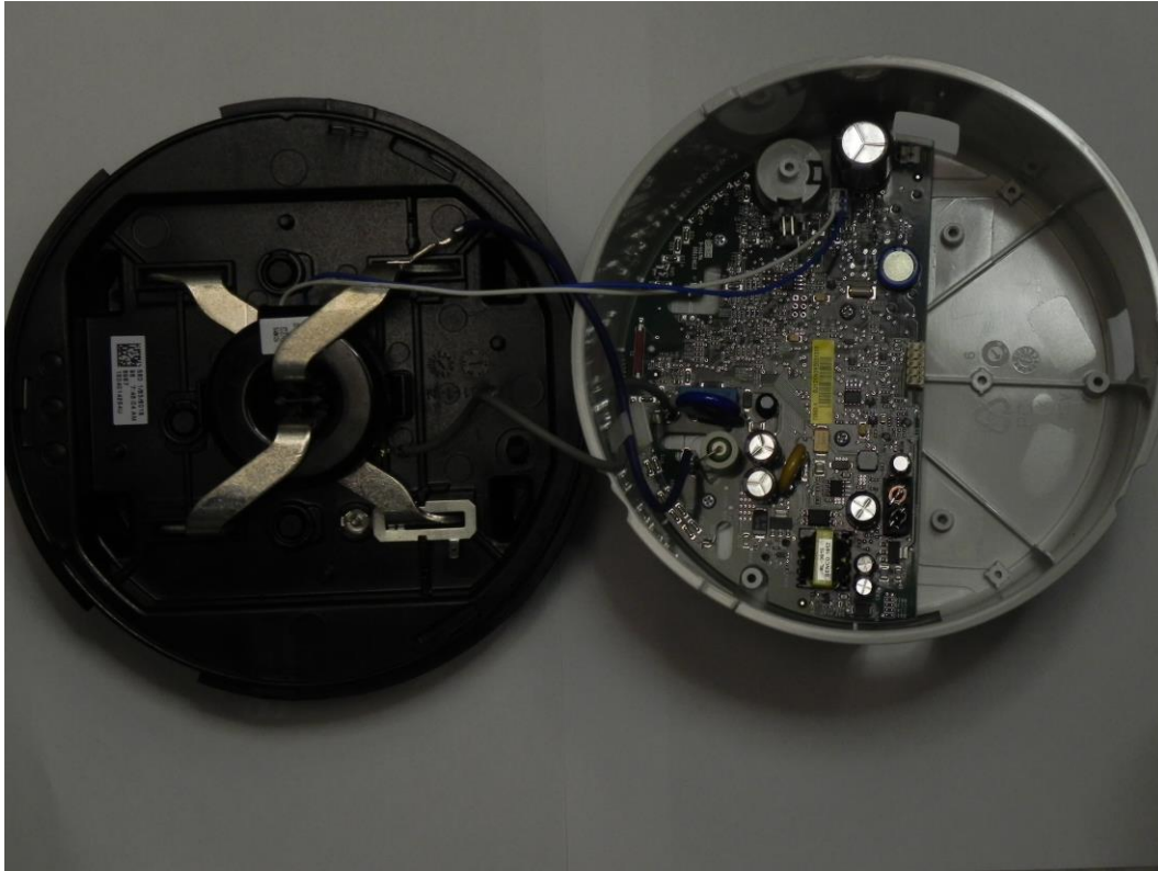
Internal View – No Communication Module Attached
