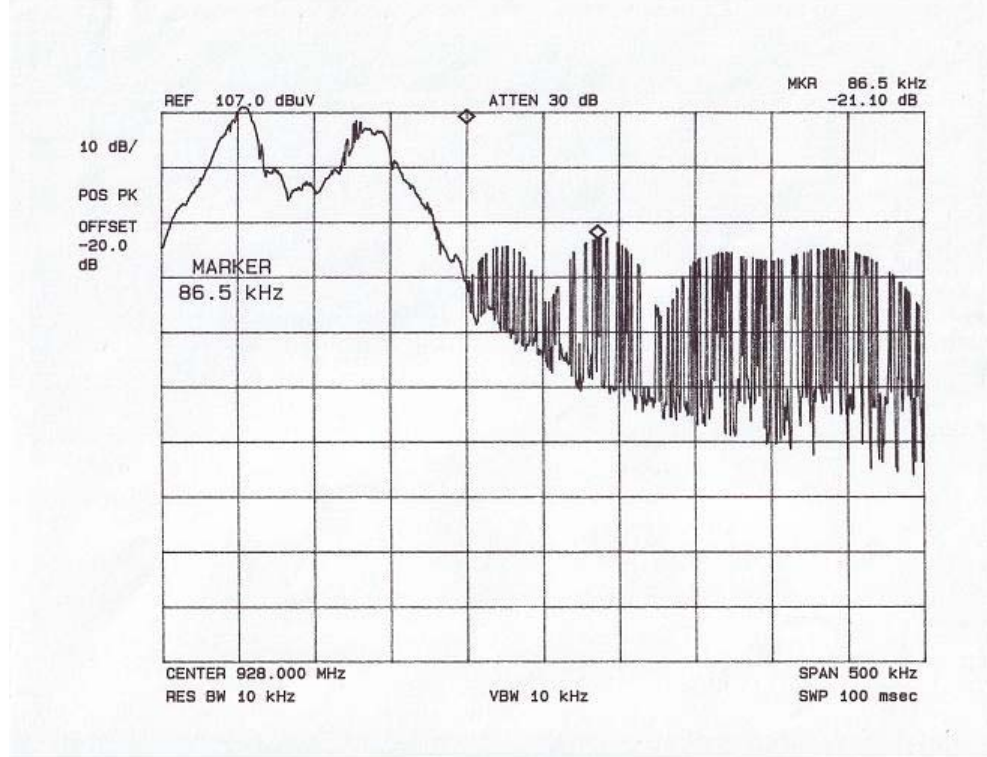
Figure 3. Upper Band-Edge
