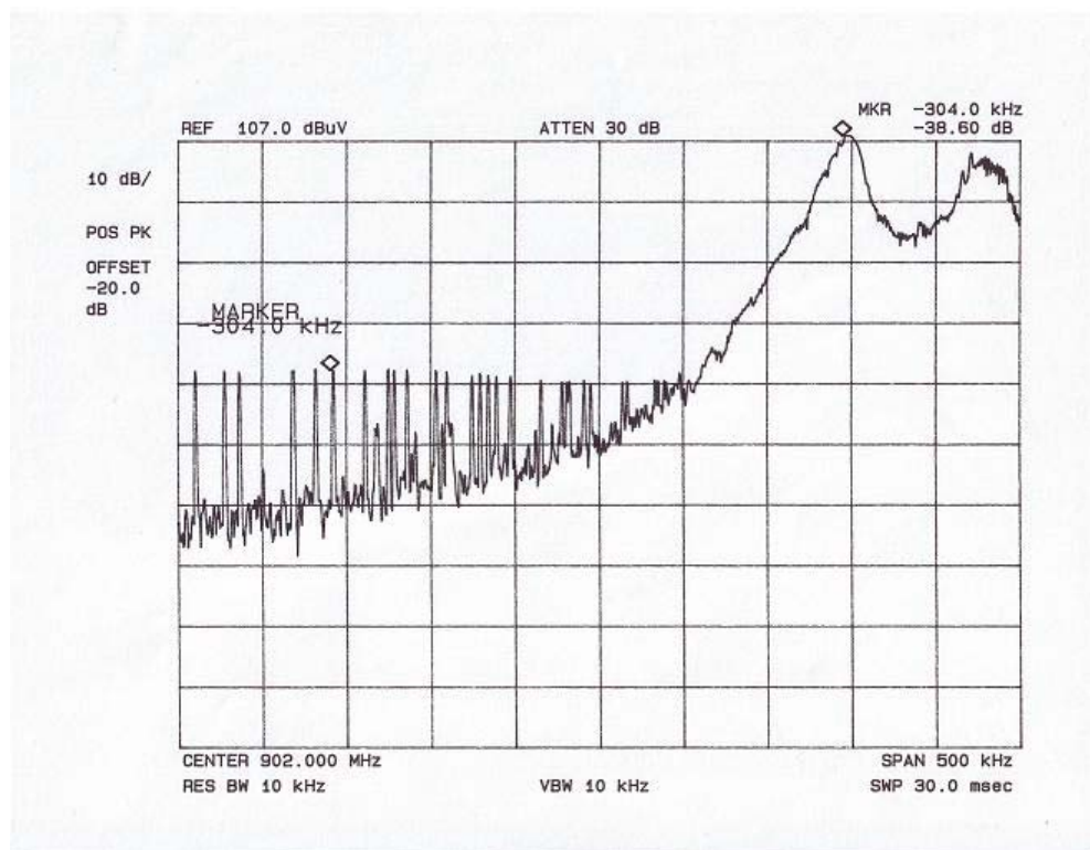
Figure 4. Lower Band-Edge
