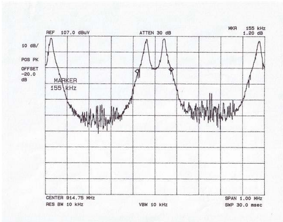
Figure 1. 20dB Bandwidth
