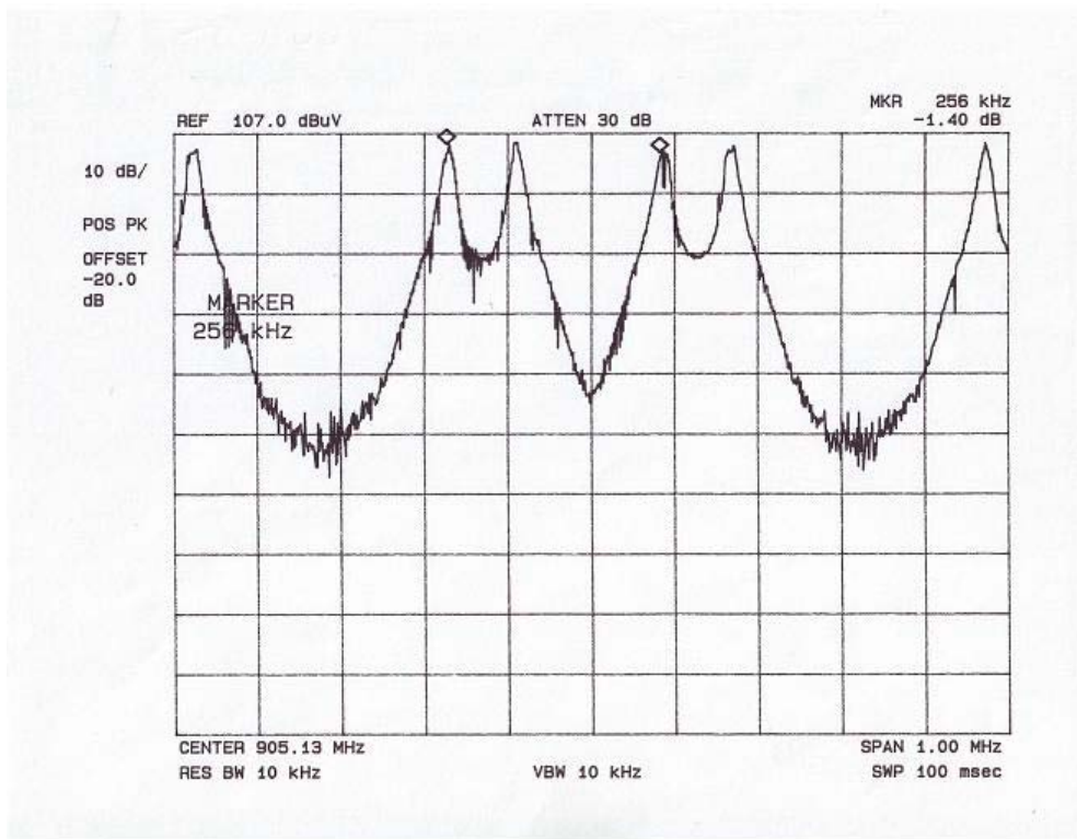
Figure 2. Channel Separation
