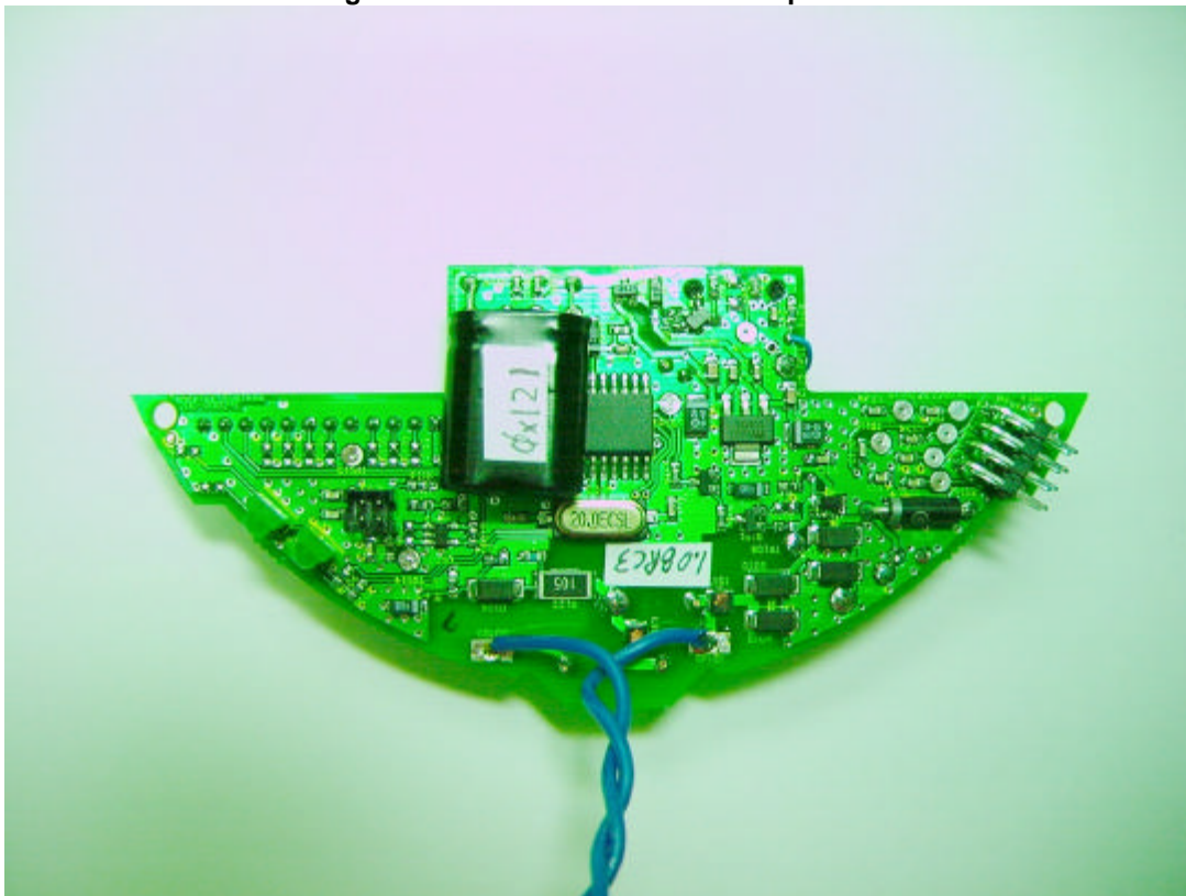
Figure 6 TC2200 Meter Host PCB Bottom side.
