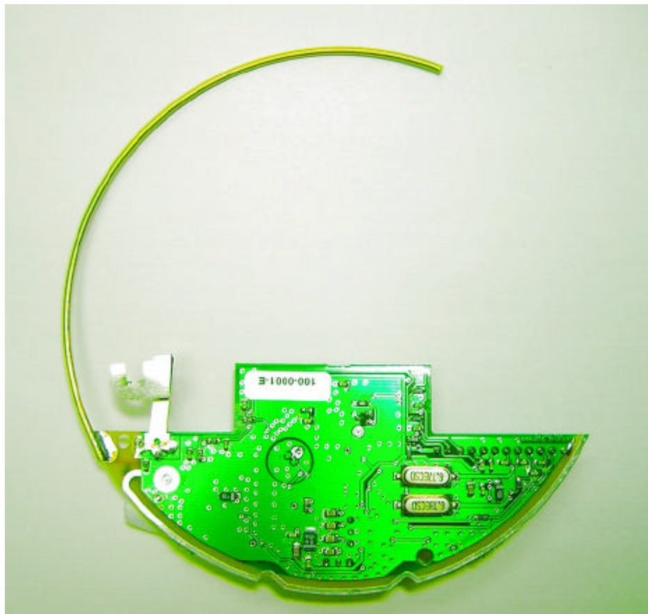
Figure 3 TC2200 Top side Transceiver PCB
