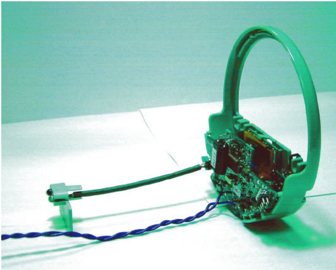
Figure 1 TC2200 Assembled in Housing with IR Port Assembly.
