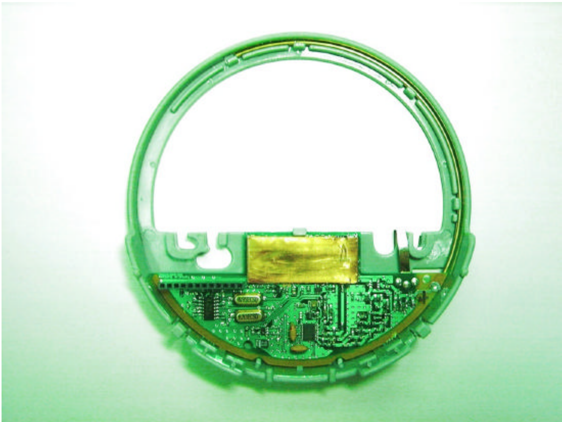
Figure 7 TC2200 Transceiver PCB inside Plastics.
