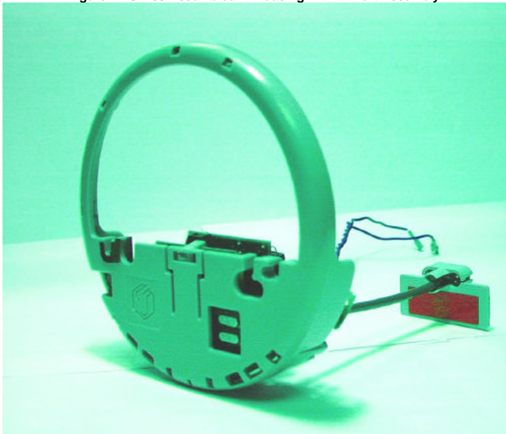
Figure 2 TC2200 Assembled in Housing with IR Port Assembly. (Front View)
