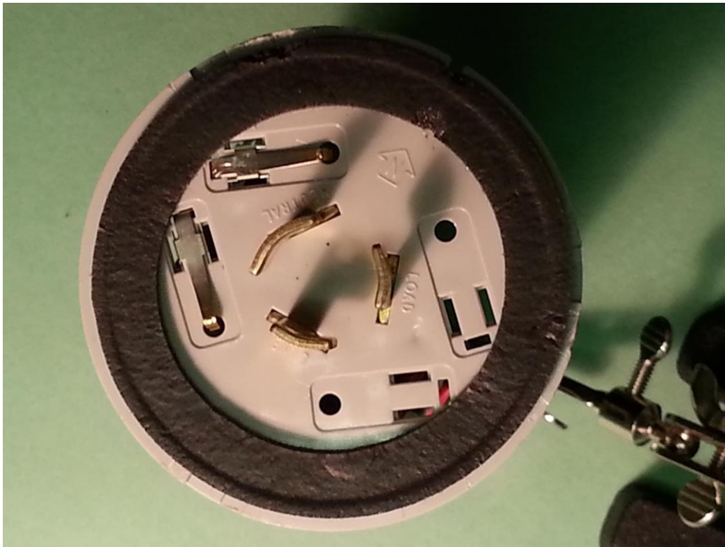
Bottom View
