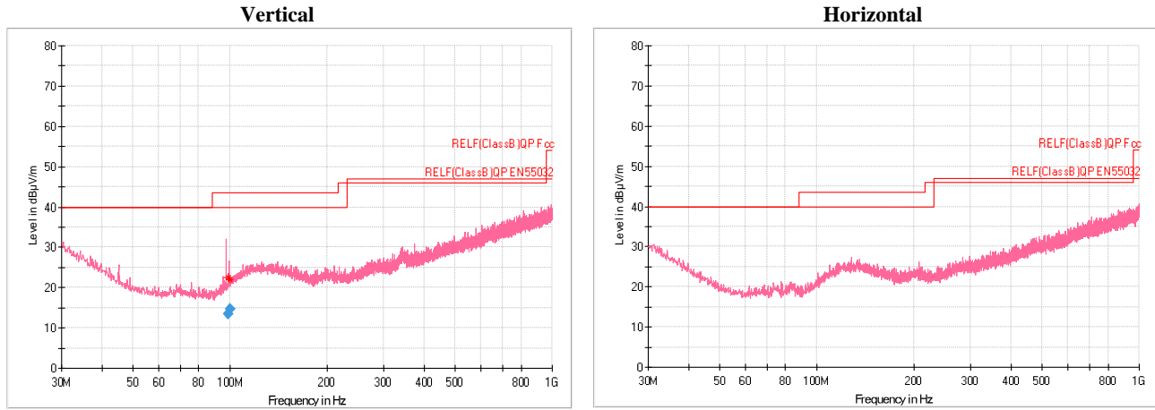
Plot 1: Radiated Emissions scanned at 3m SAC—for reference only
