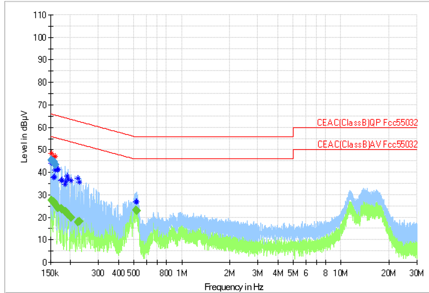
Plot 2: Conducted Emissions –120Vac/60Hz, Line 1—for reference only
