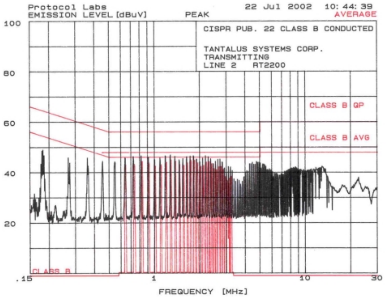
Transmitting Line 2
