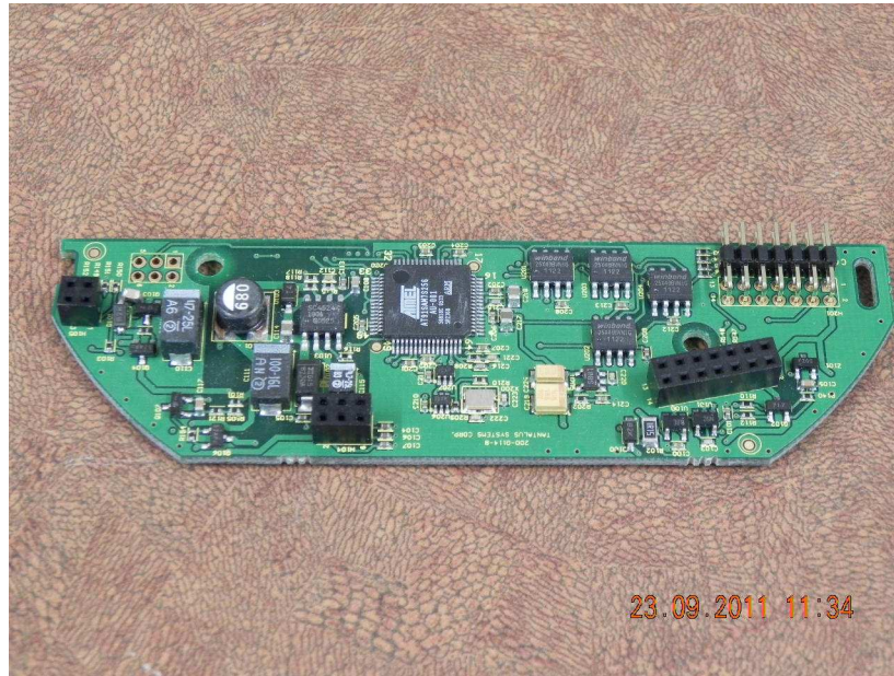
PP1316 PCB1 – Front View
