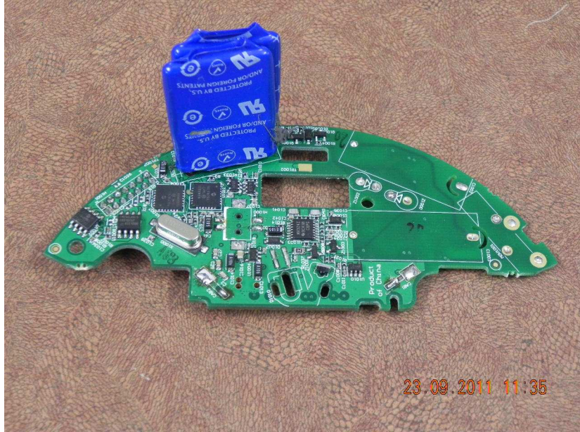
PP1316 PCB3 – Top View
