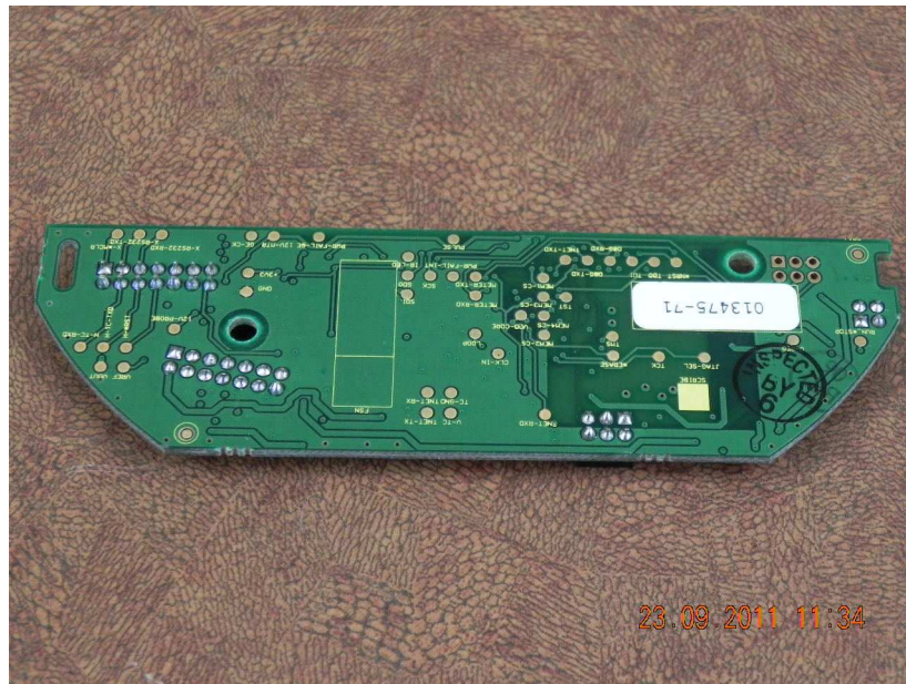
PP1316 PCB1 – Bottom View
