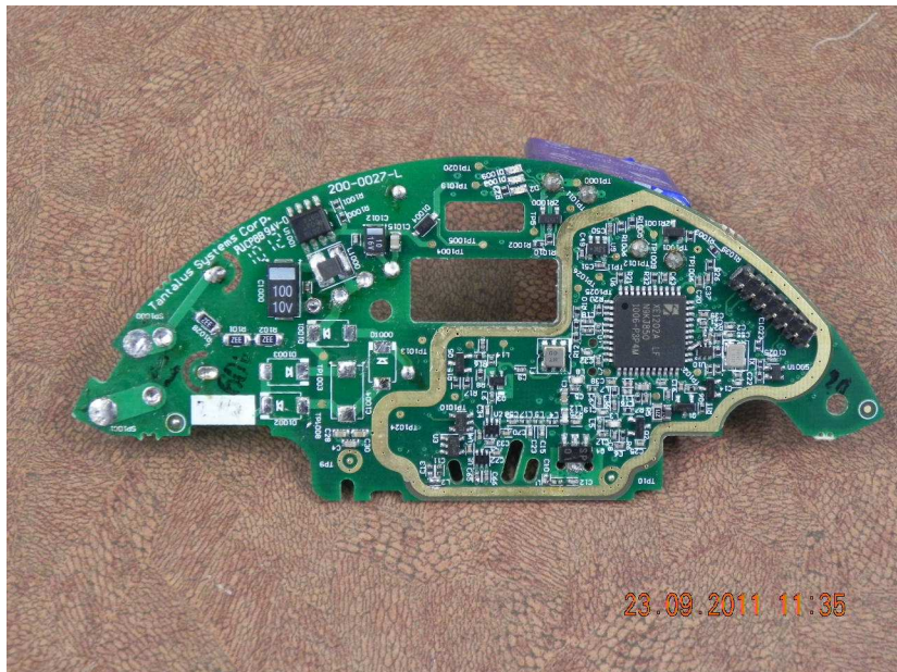
PP1316 PCB3 – Bottom View
