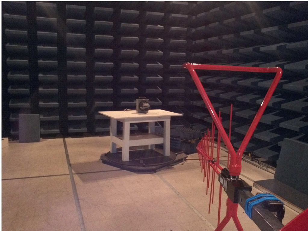
Emissions Test Setup – Unintentional Radiated Emissions
